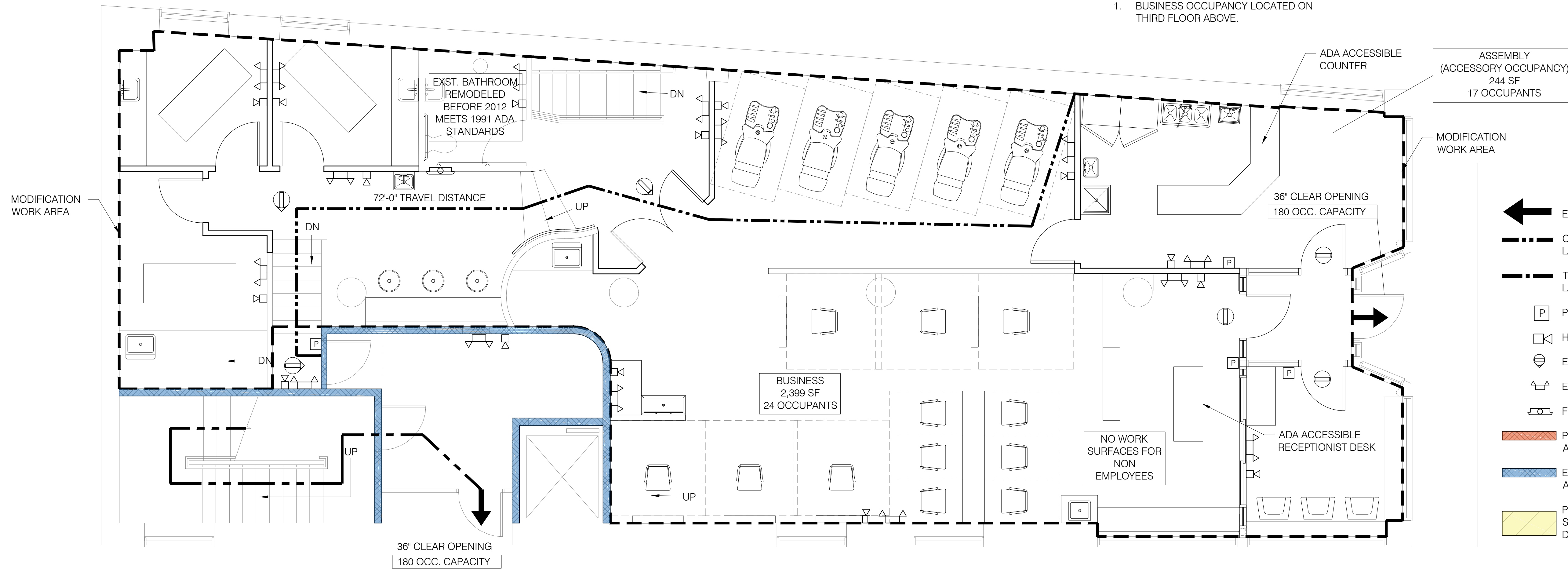
1 FIRST FLOOR LIFE SAFETY PLAN SCALE: 1/4" = 1'-0"
