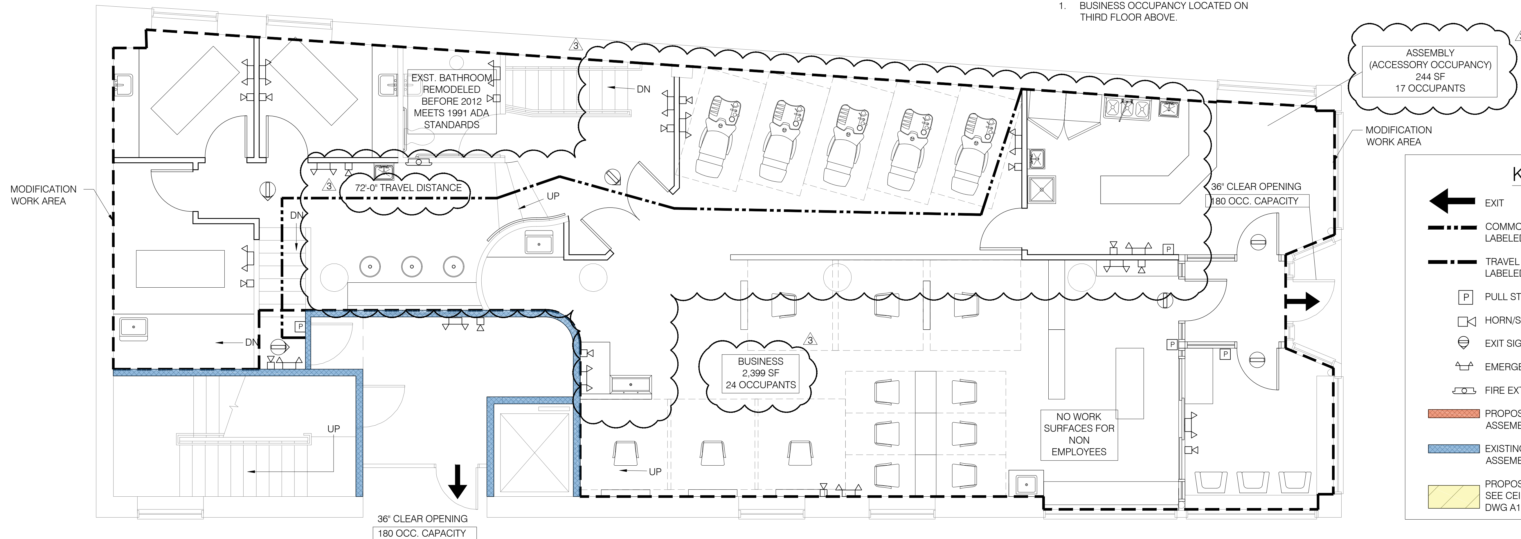
1 FIRST FLOOR LIFE SAFETY PLAN SCALE: 1/4" = 1'-0"
