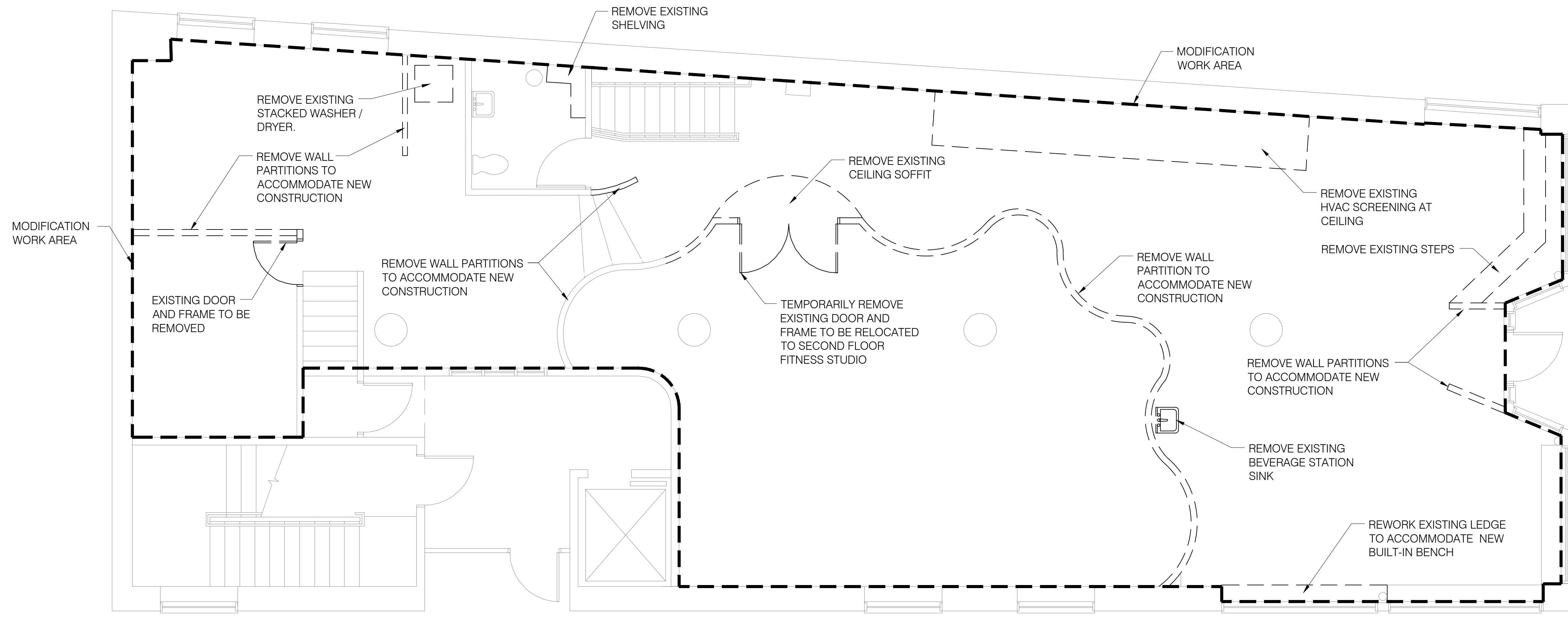
2 0 4'-0" SCALE: 1/4" = 1'-0" FIRST FLOOR DEMOLITION PLAN
