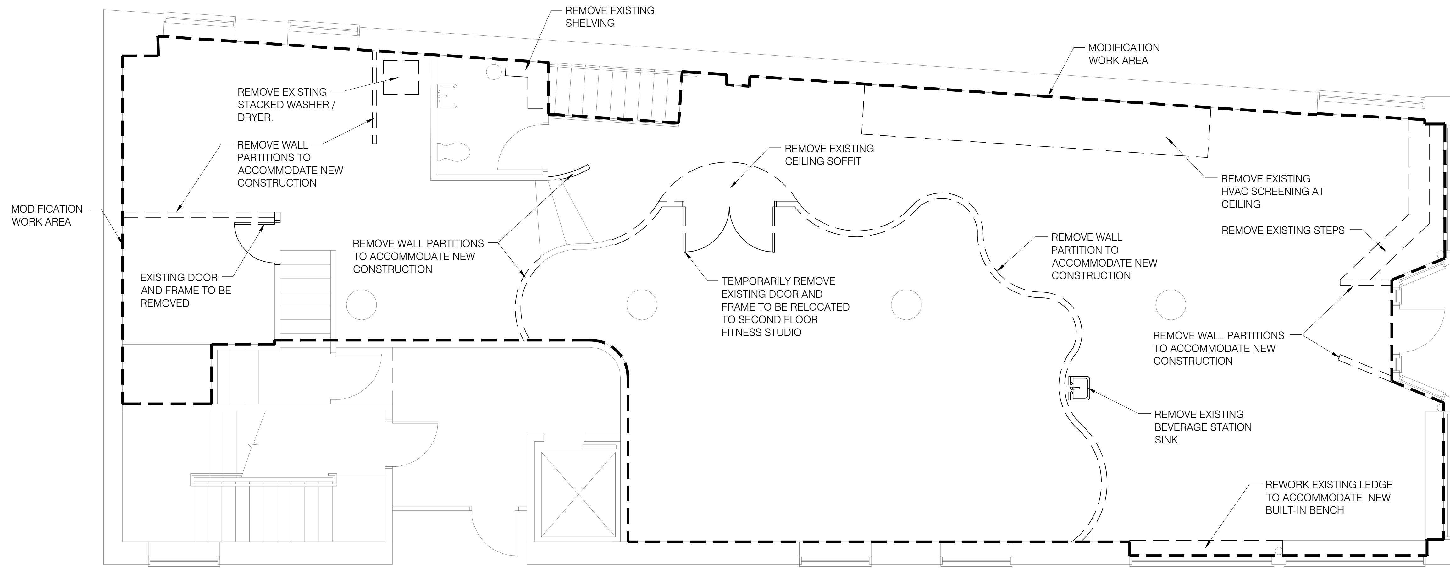
FIRST FLOOR DEMOLITION PLAN SCALE: 1/4" = 1'-0" 0 4'-0"
