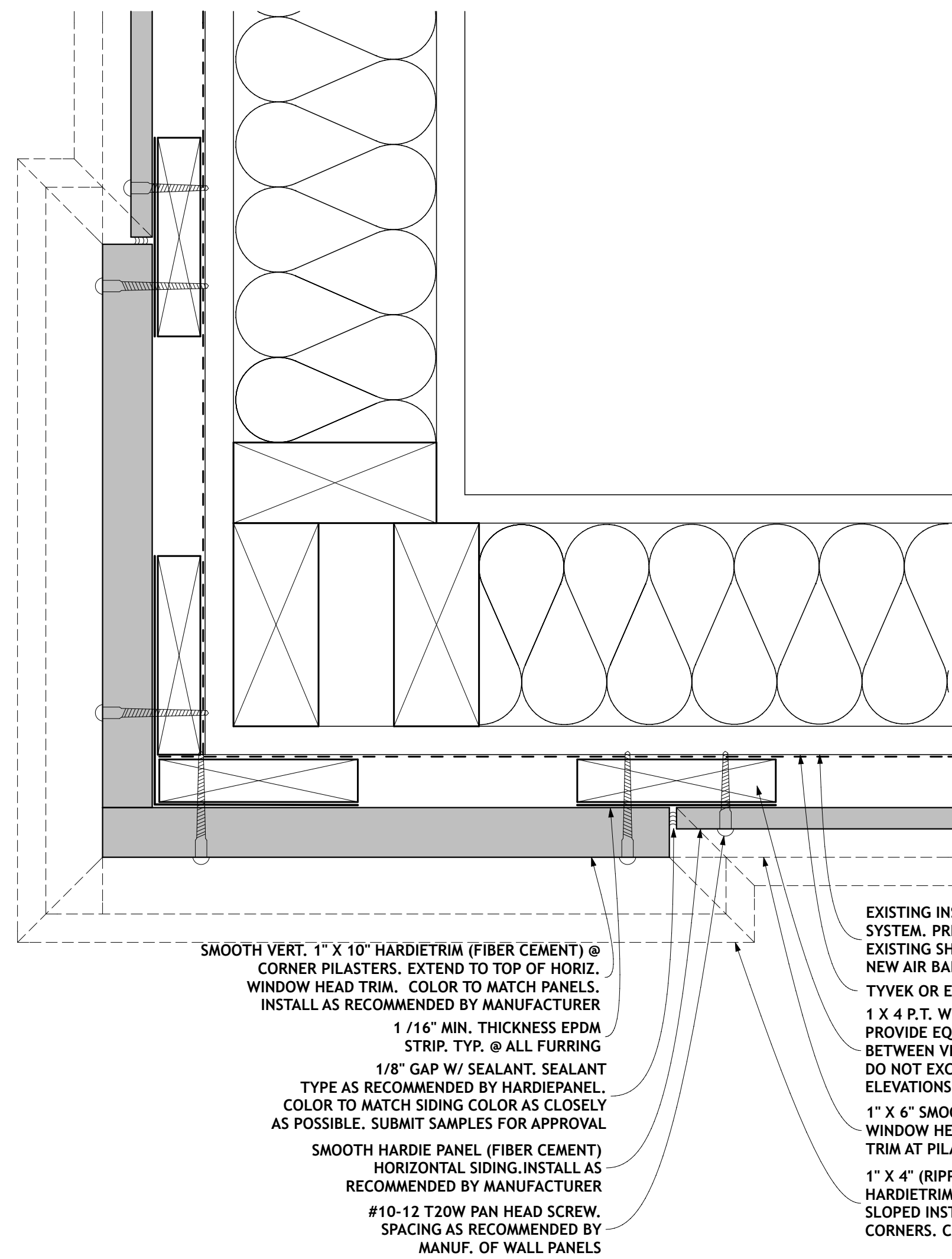
5 PLAN DETAIL- CORNER PILASTER SCALE: 6" = 1'-0"
