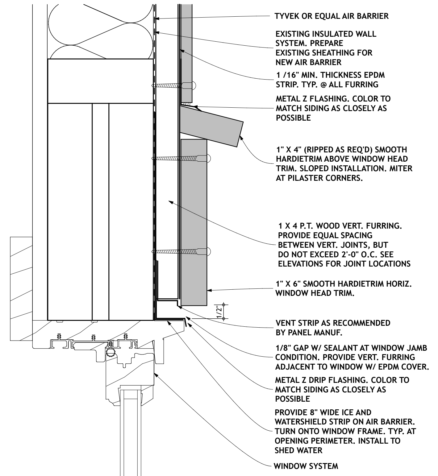
4 SECTION DETAIL- WINDOW HEAD TRIM SCALE: 6" = 1'-0"
