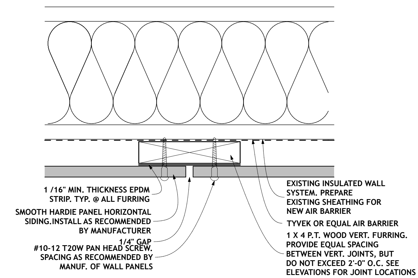
6 PLAN DETAIL- VERT. PANEL JOINT SCALE: 6" = 1'-0"
