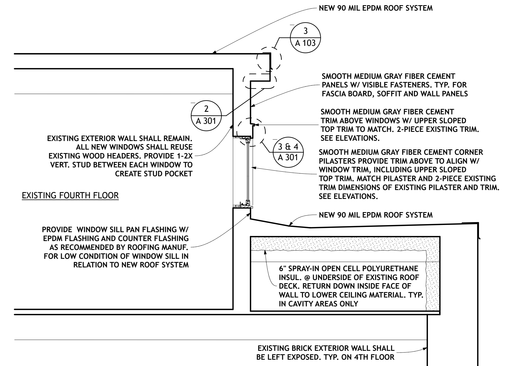
1 PARTIAL BUILDING SECTION SCALE: 1/2" = 1'-0"
