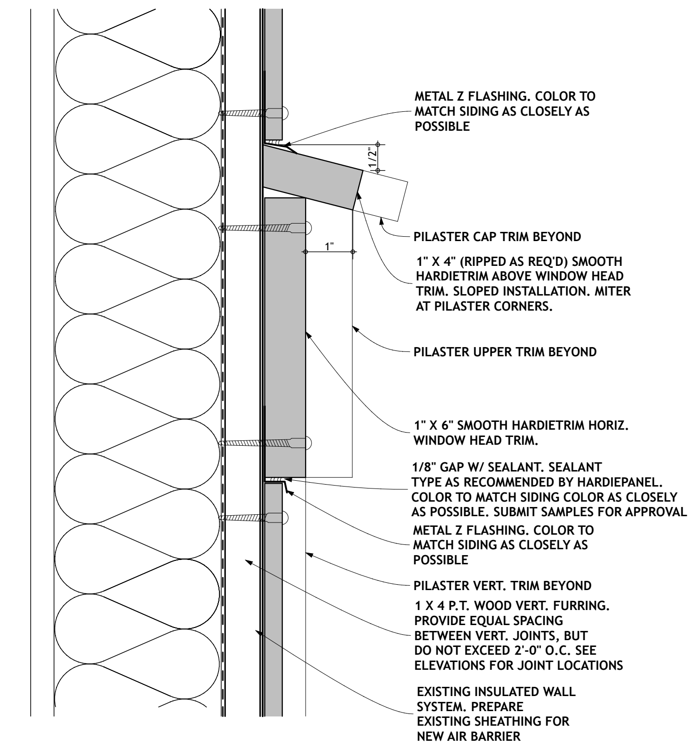
3 SECTION DETAIL- HEAD TRIM TO PANEL SCALE: 6" = 1'-0"
