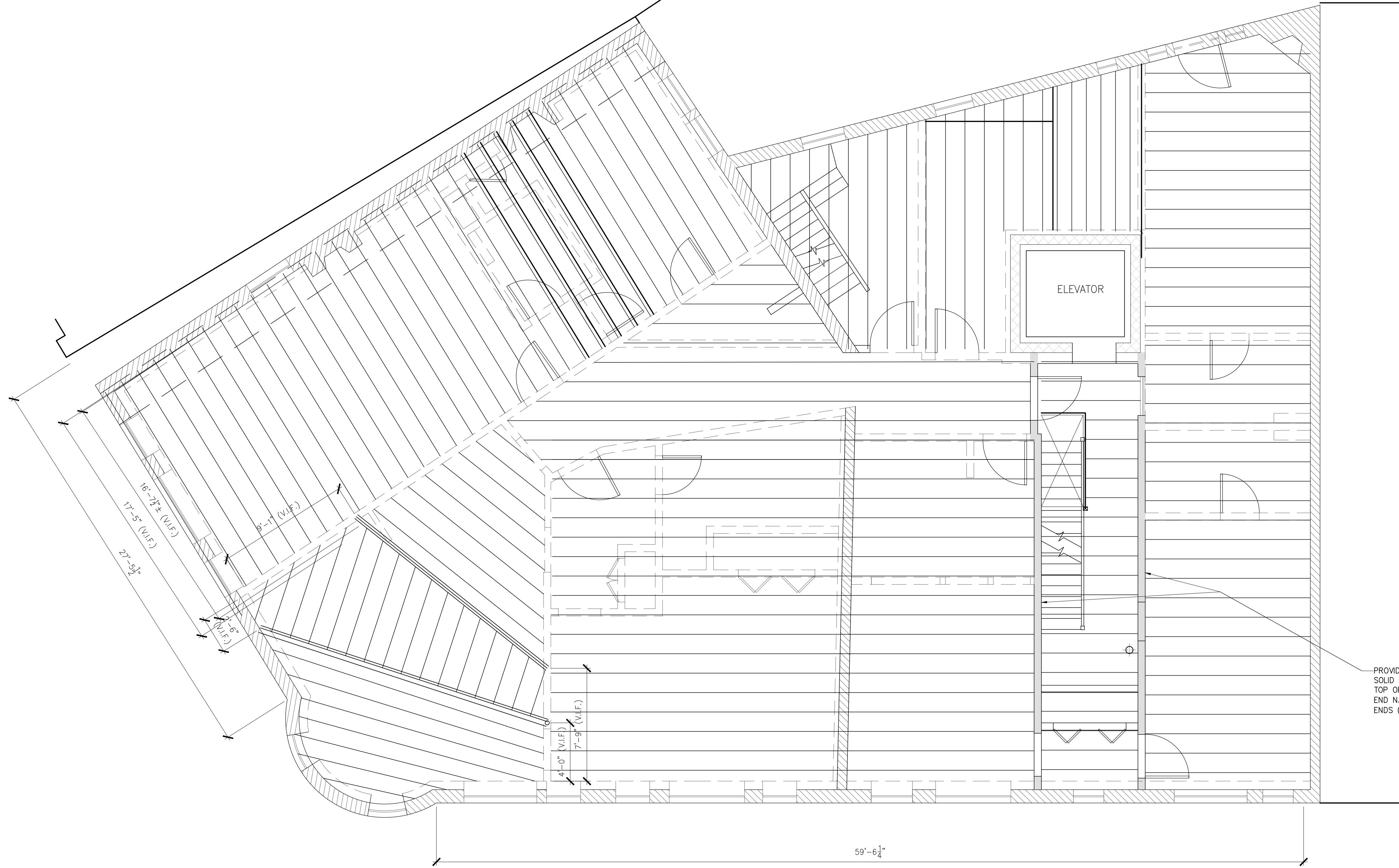
THIRD FLOOR FRAMING PLAN 1/4" = 1'-0"
