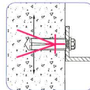
SLEEVE-ANCHOR MOUNTING DETAIL NOT TO SCALE
