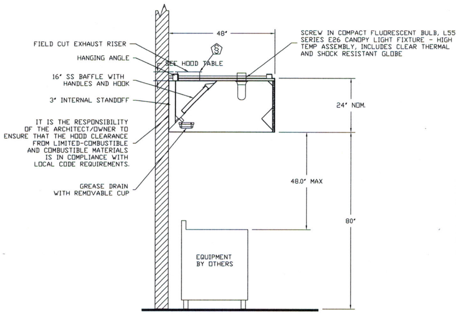
SECTION VIEW - MODEL 4824ND-2 HOOD - #1
