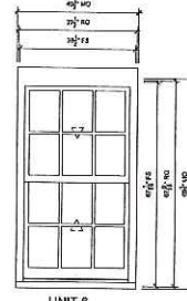
UNIT 6 SCALE: 3/4\"/>
