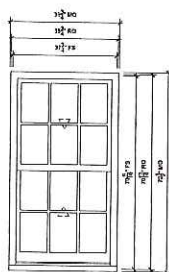
UNIT 3 SCALE: 3/4\"/>
