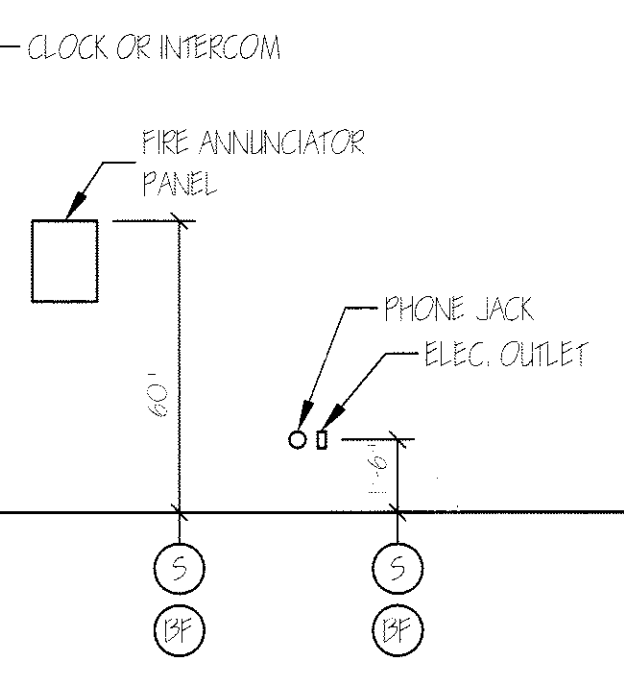
ELECTRICAL & FIRE PROTECTION DEVICES TYPICAL UNLESS NOTED OTHERWISE NTS
