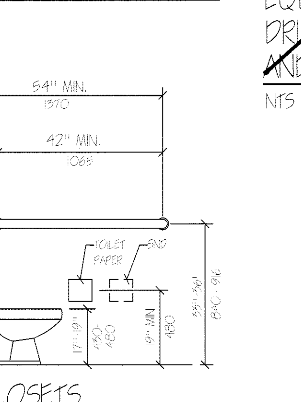
NOT USED GRAB BARS AT WATER CLOSETS NTS
