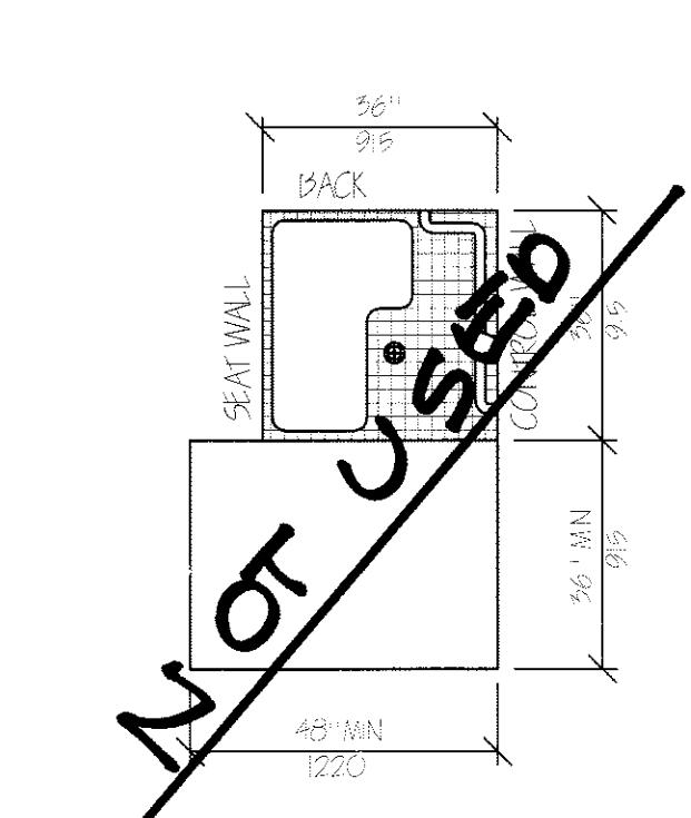
NOT USED SHOWER SEAT DESIGN NTS
