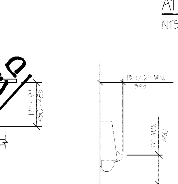
NOT USED HEIGHT AND DEPTH OF URINALS NTS
