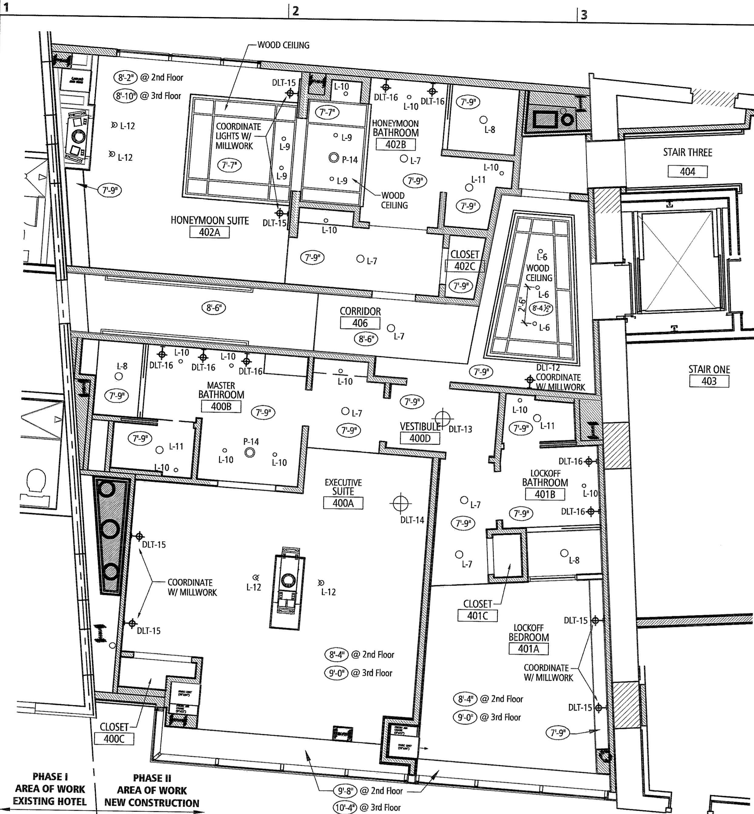
1 Second Floor Reflected Ceiling Plan Scale: 1/4" = 1'-0" NOTE: Third Floor Similar
