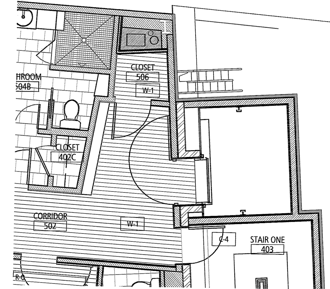
3 Partial Third Floor Finish Plan Scale: 1/4" = 1'-0"
