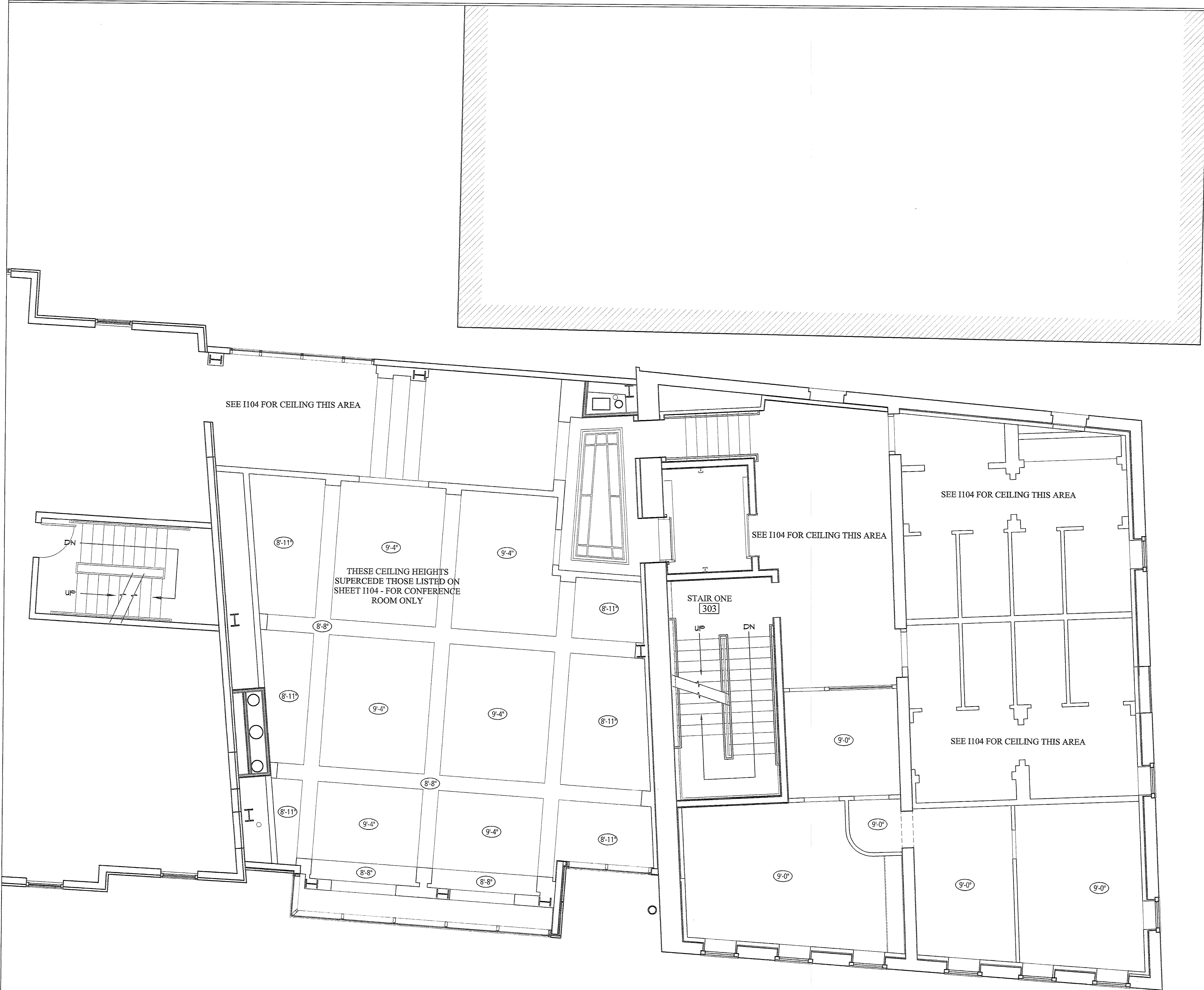
3 | FIRST FLOOR REFLECTED CEILING PLAN SCALE: 1/4" = 1'-0"
