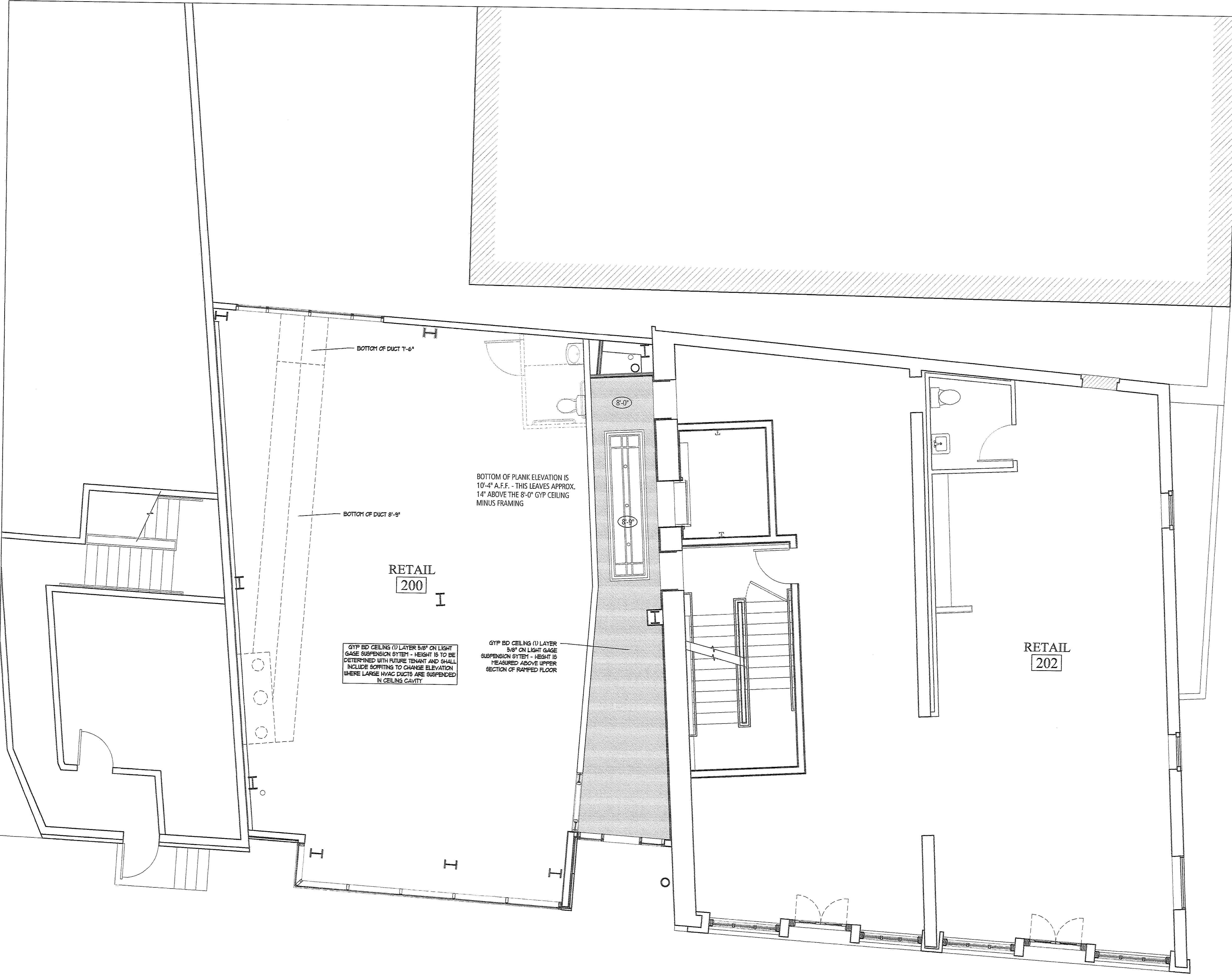
1 | GROUND FLOOR REFLECTED CEILING PLAN SCALE: 1/4" = 1'-0"
