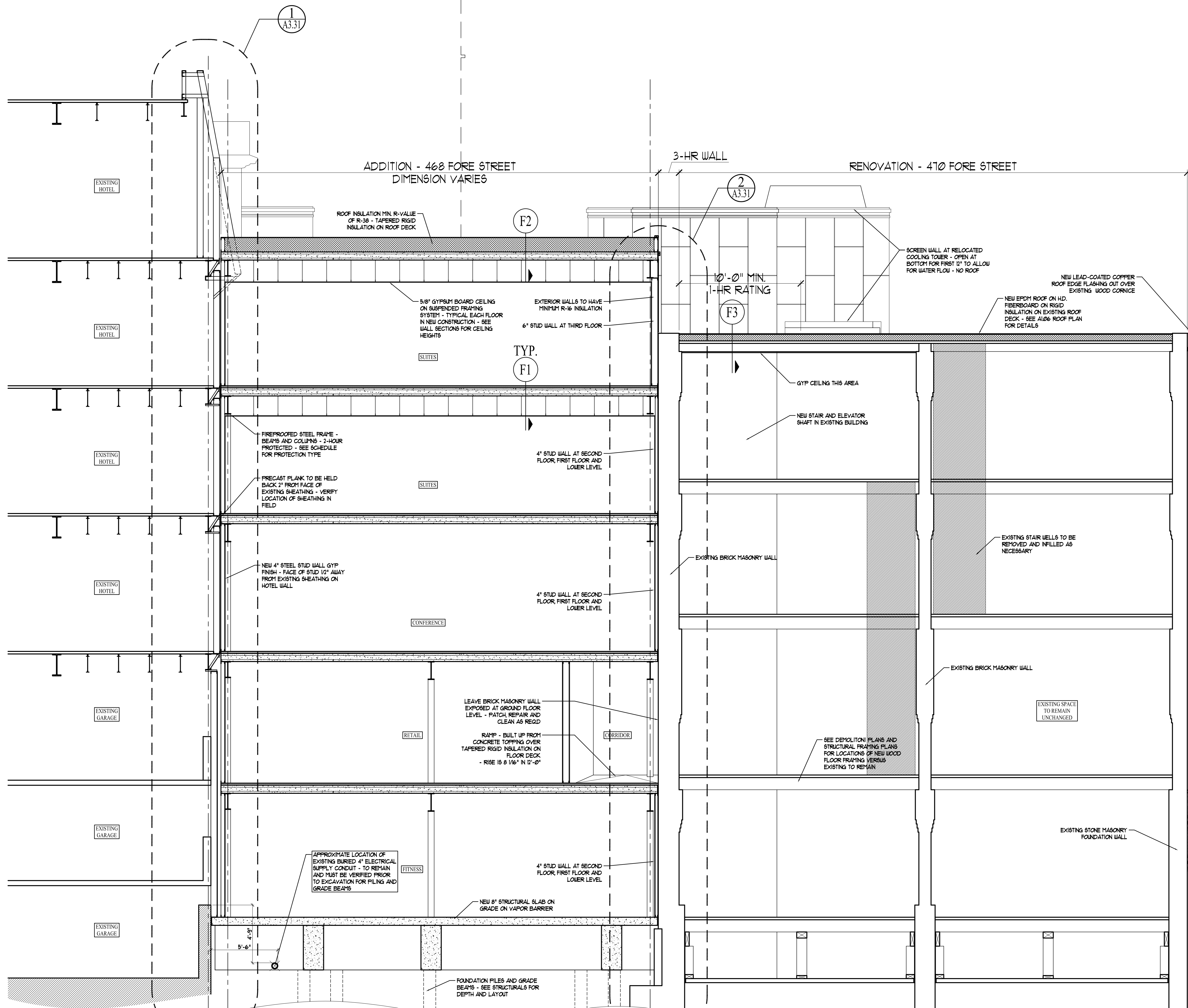
BUILDING SECTION SCALE: 1/4"=1'-0"
