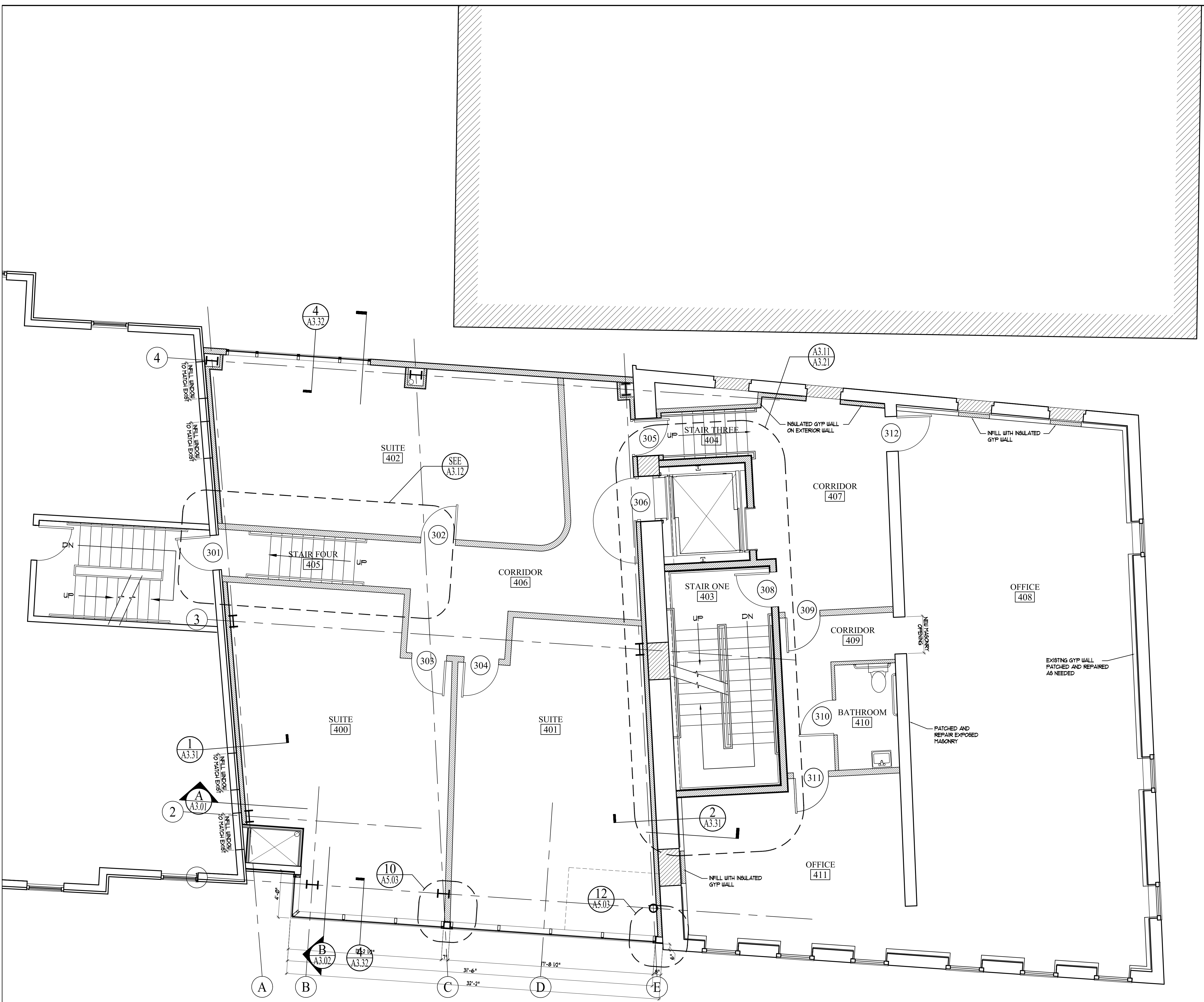
4 SECOND FLOOR PLAN SCALE: 1/4"=1'-0"
