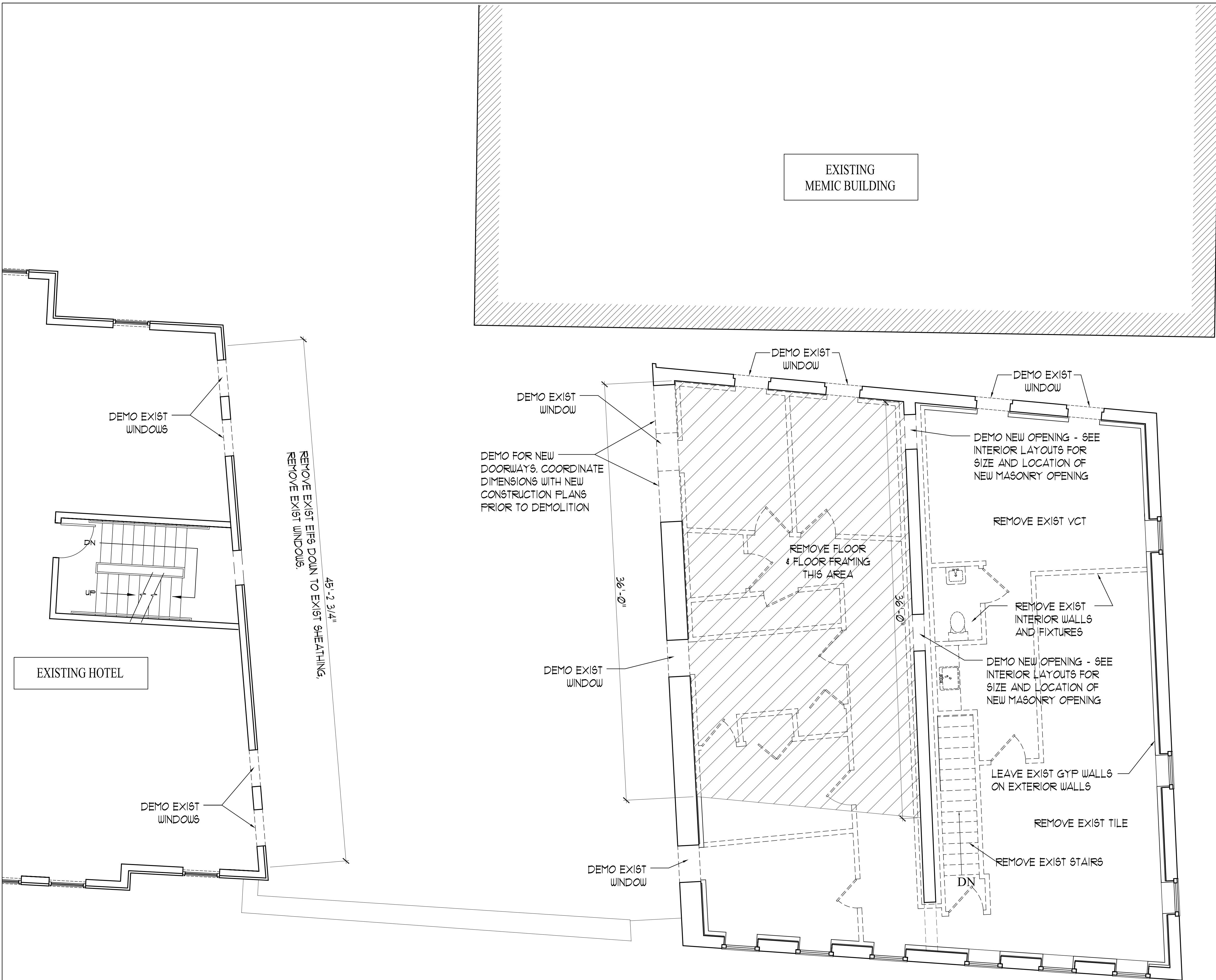
4 SECOND FLOOR DEMOLITION PLAN SCALE: 1/4"=1'-0"
