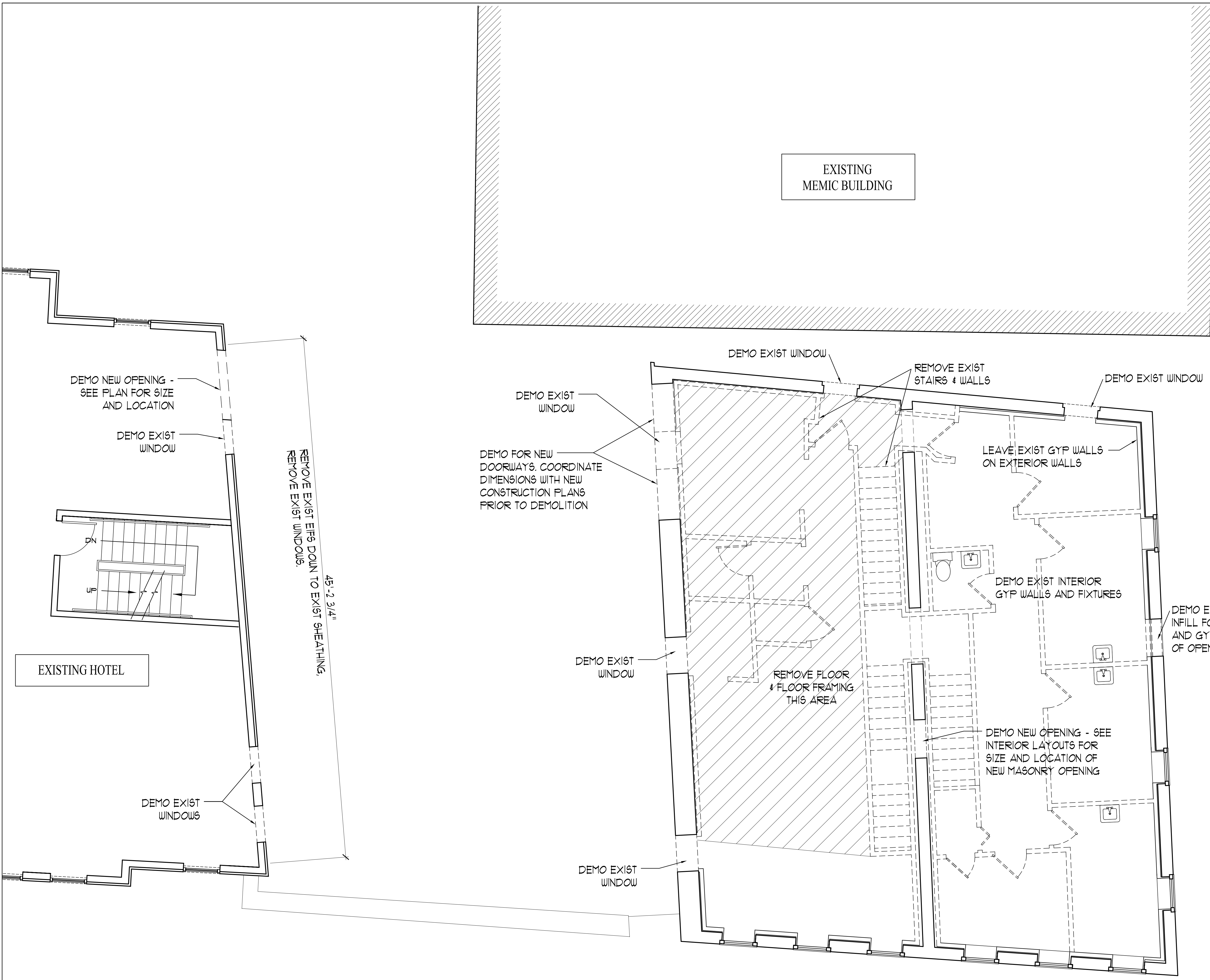
3 | FIRST FLOOR DEMOLITION PLAN SCALE: 1/4" = 1'-0"
