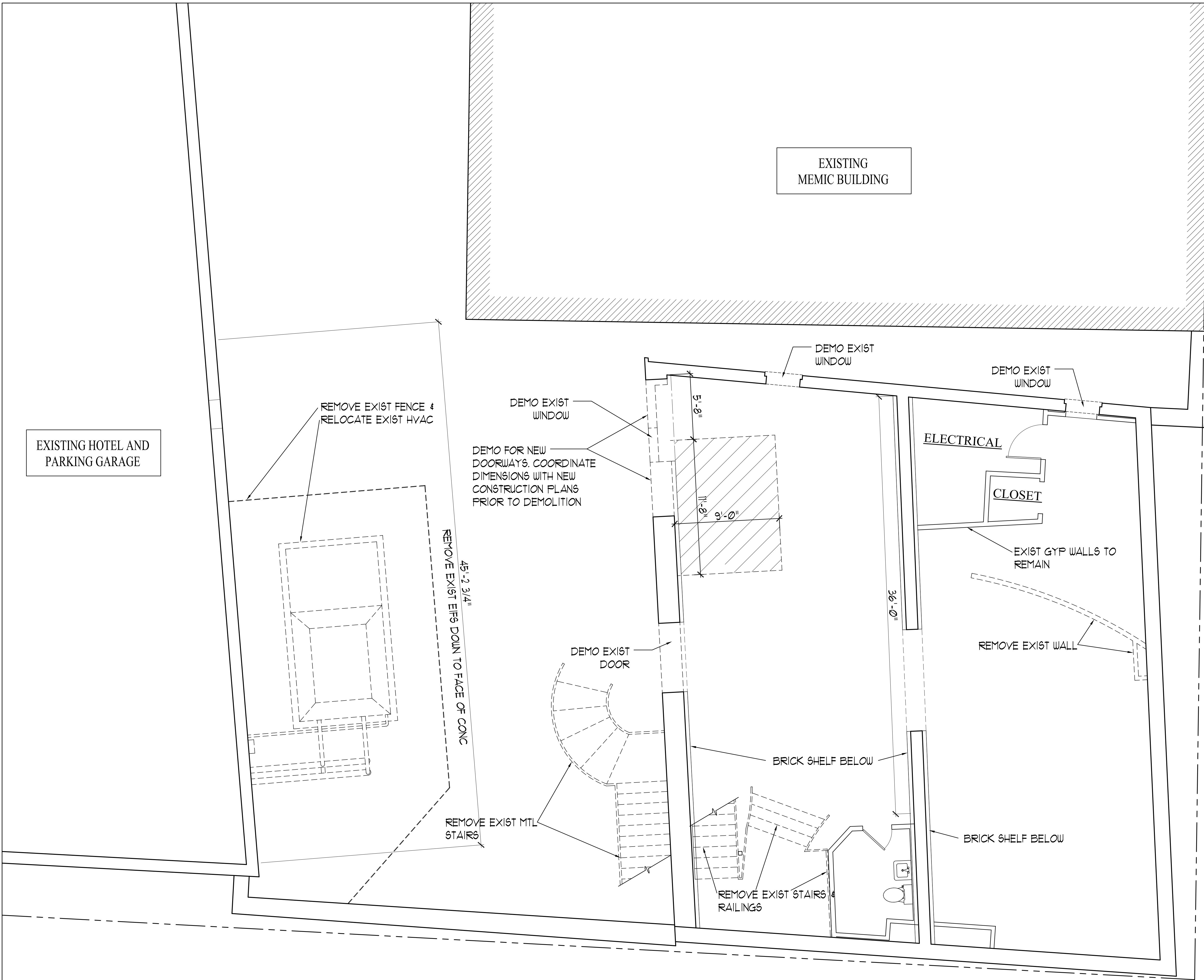
LOWER LEVEL DEMOLITION PLAN SCALE: 1/4" = 1'-0"
