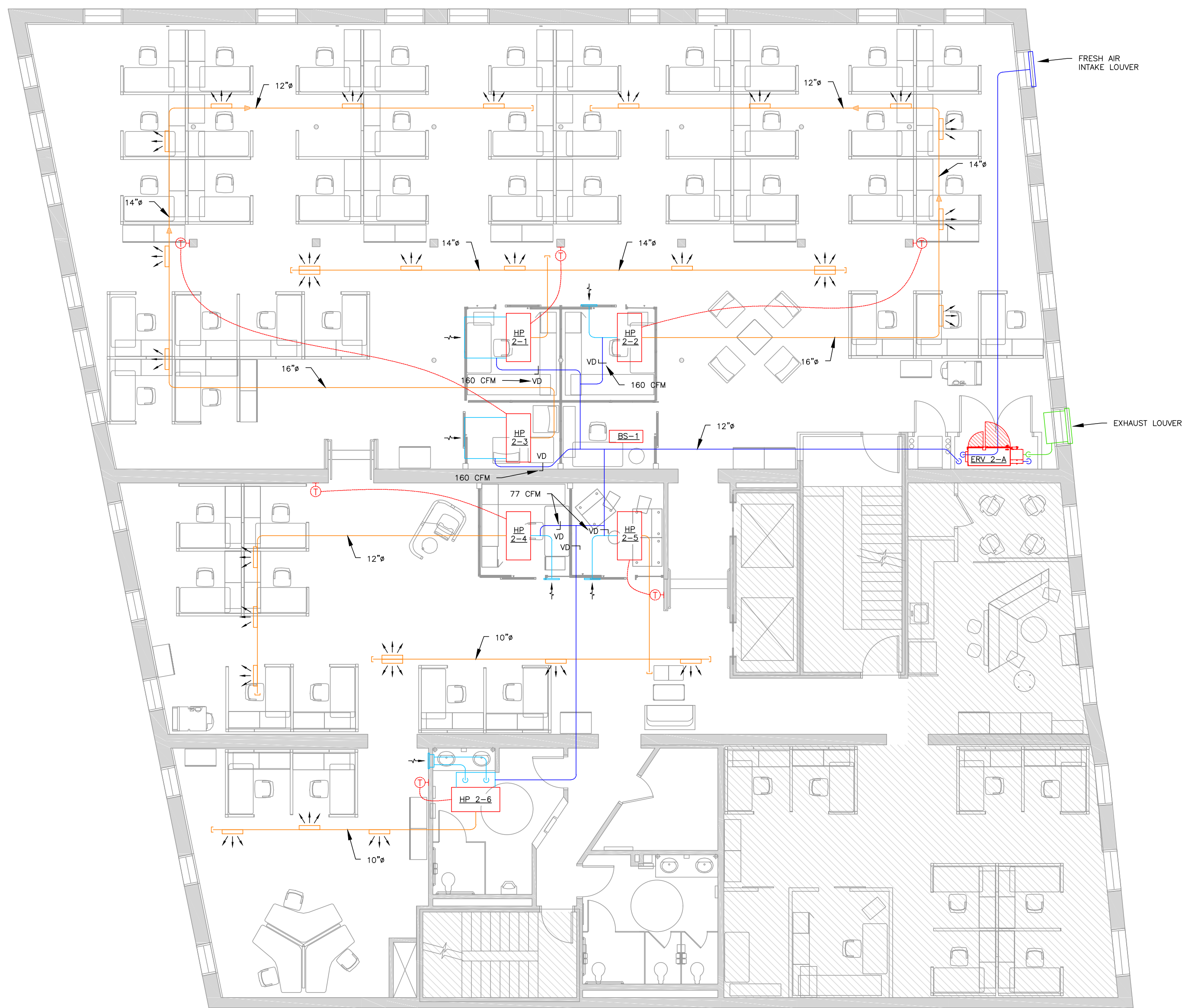
SECOND FLOOR HVAC PLAN SCALE: 1/8" = 1'-0"
