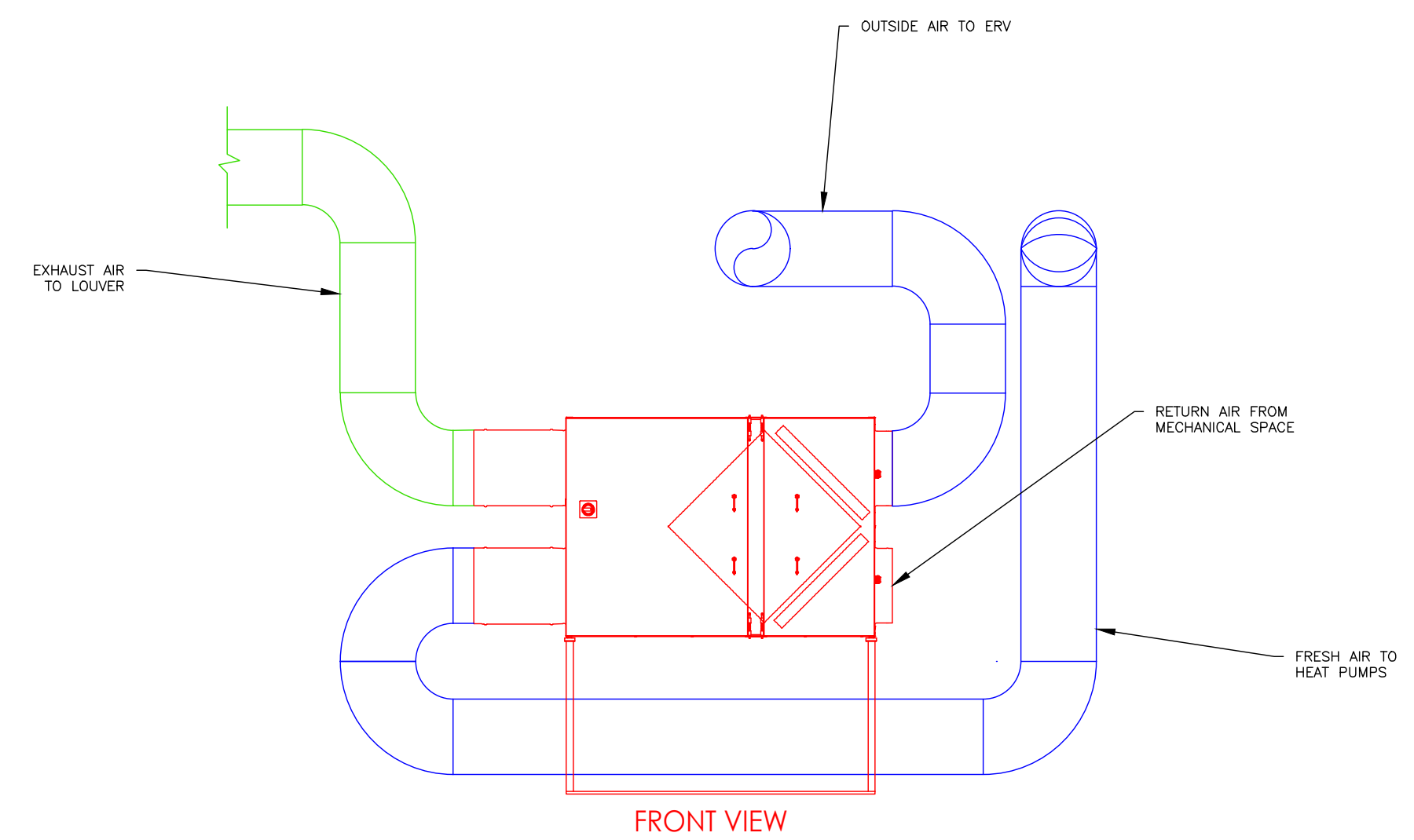
ERV DETAIL FRONT VIEW SCALE: NOT TO SCALE
