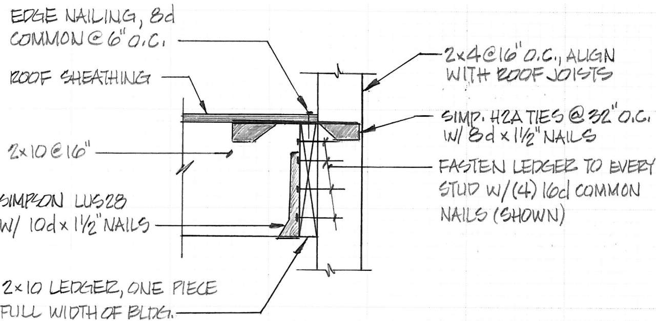
2 LEDGER SECTION DETAIL @ ROOF S-2.2 SCALE: 1 1/2" = 1'-0"
