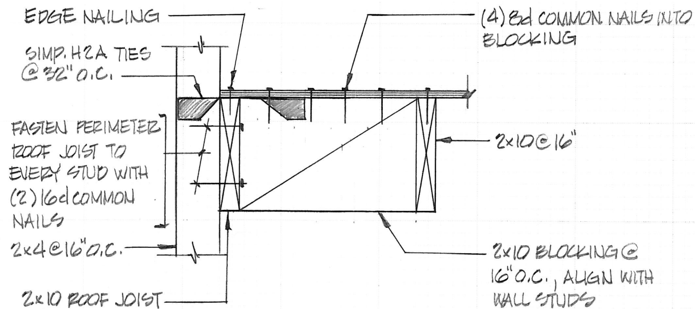
3 ROOF SECTION @ NORTH AND SOUTH WALLS S-2.2 SCALE: 1 1/2" = 1'-0"
