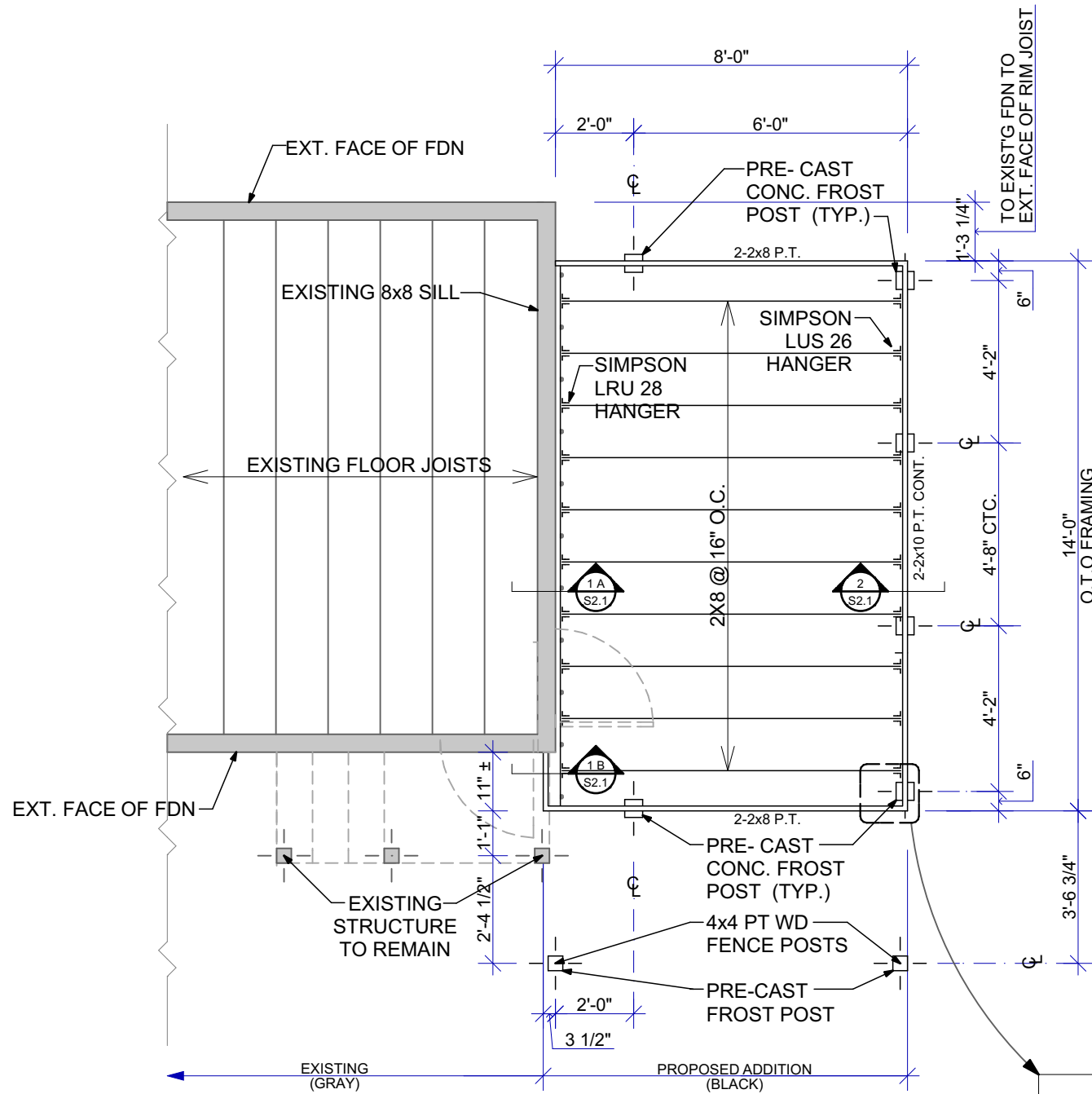
1 S-1.1 1st FLOOR FRAMING PLAN SCALE: 1/4" = 1'-0"
