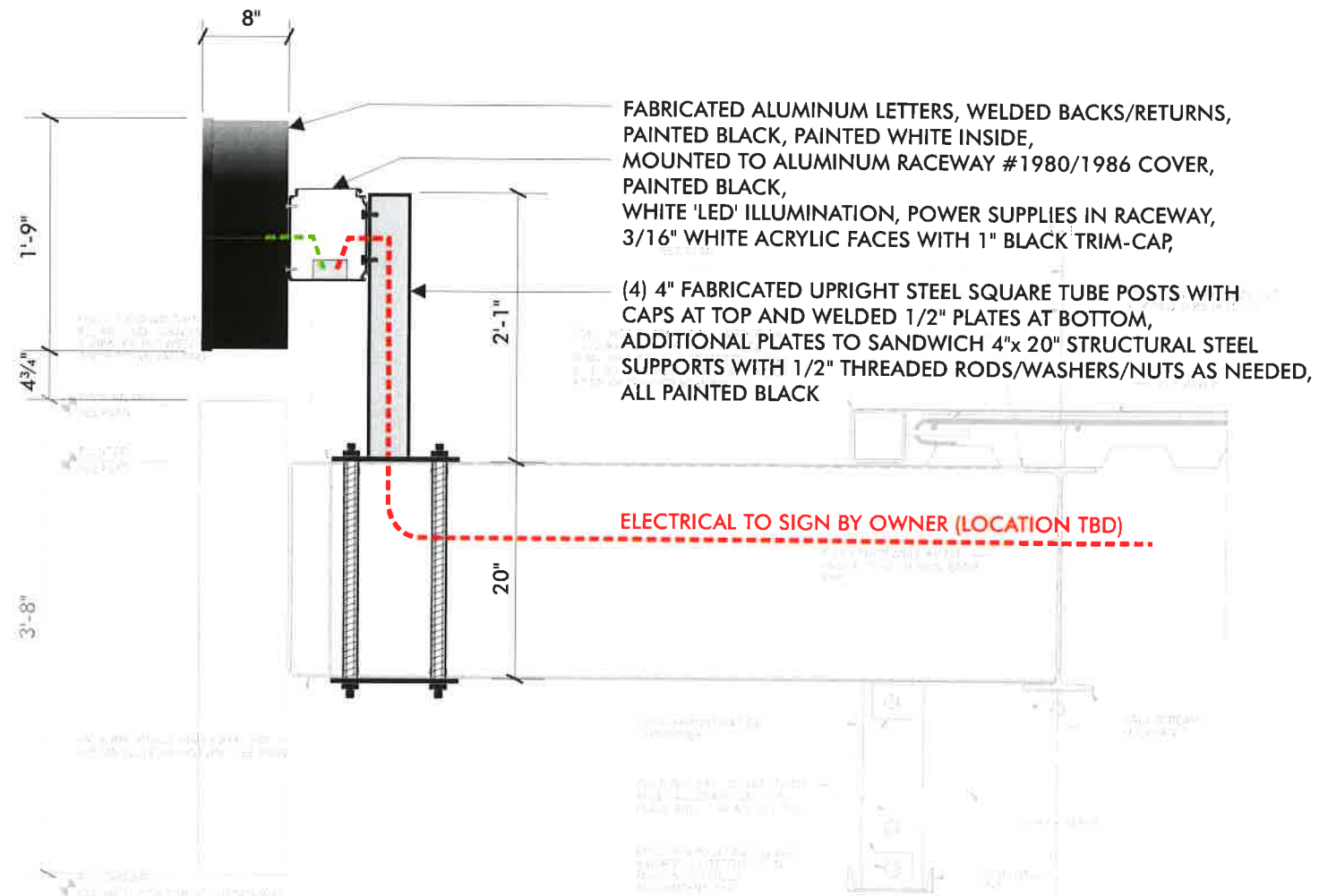
END VIEW
