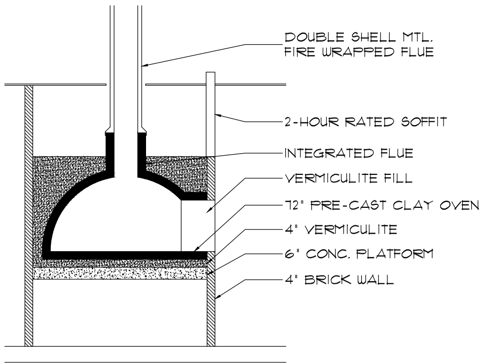
BRICK OVEN SECTION SCALE: 1/4" = 1'-0"
