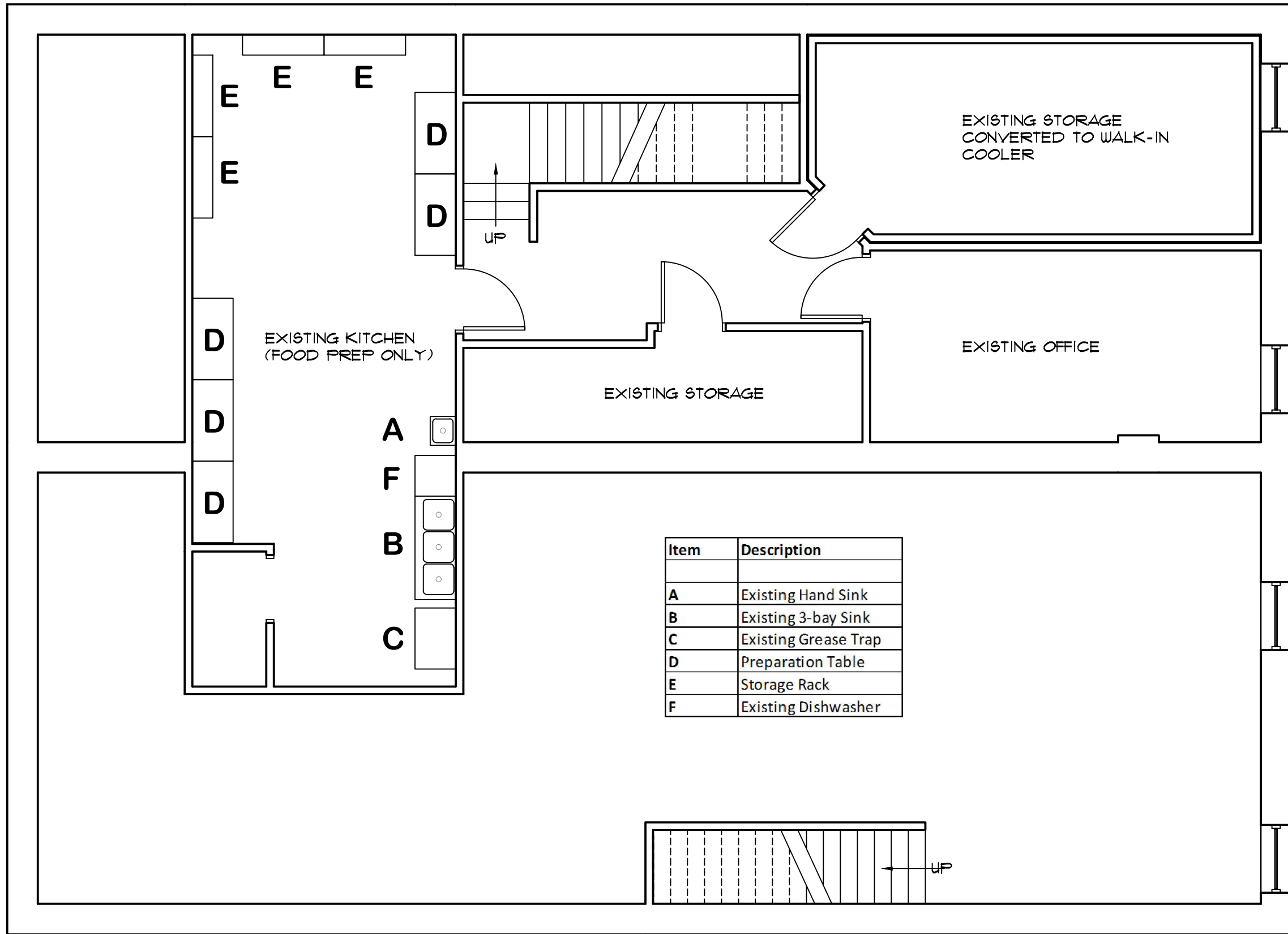
EXISTING/REVISED FLOOR PLAN SCALE: 3/16" = 1'-0"
