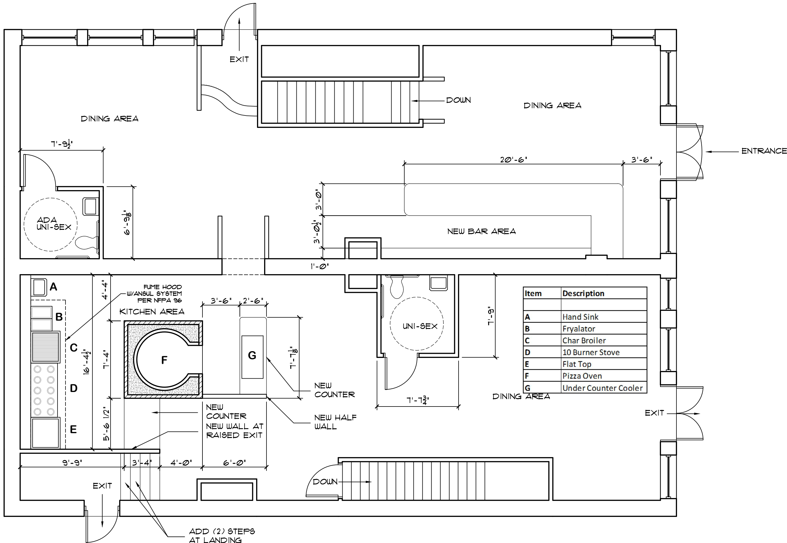
REVISED FLOOR PLAN SCALE: 3/16" = 1'-0"
