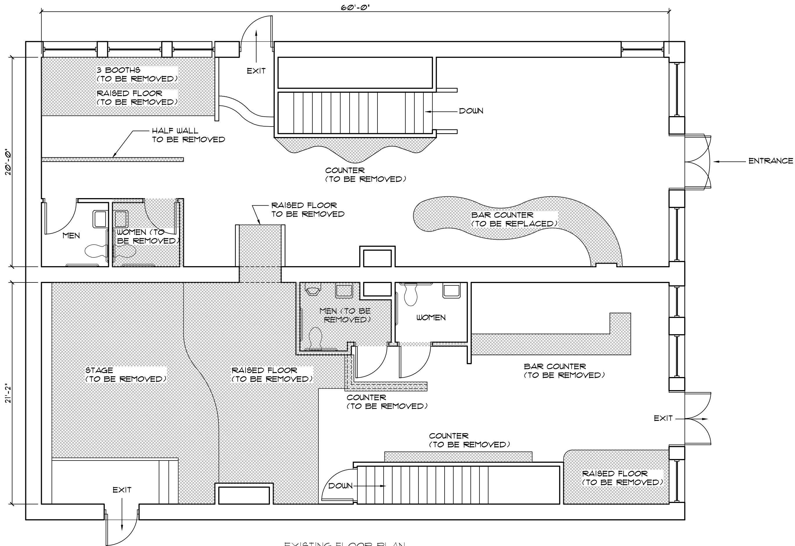
EXISTING FLOOR PLAN SCALE: 3/16" = 1'-0"
