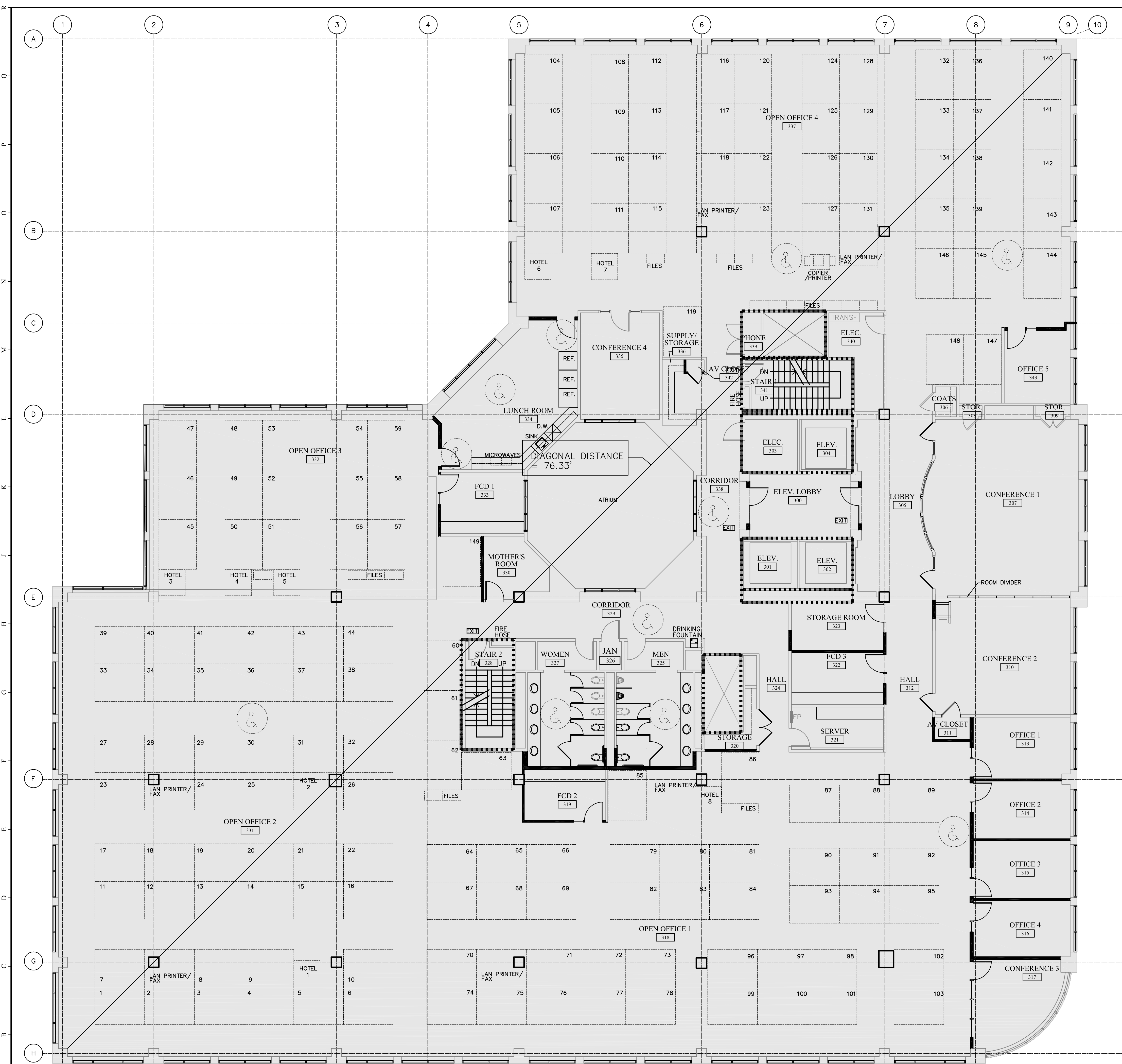
A1 THIRD FLOOR PLAN
