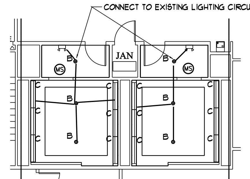
FOURTH FLOOR PARTIAL LIGHTING PLAN SCALE - 1/8" = 1'-0"
