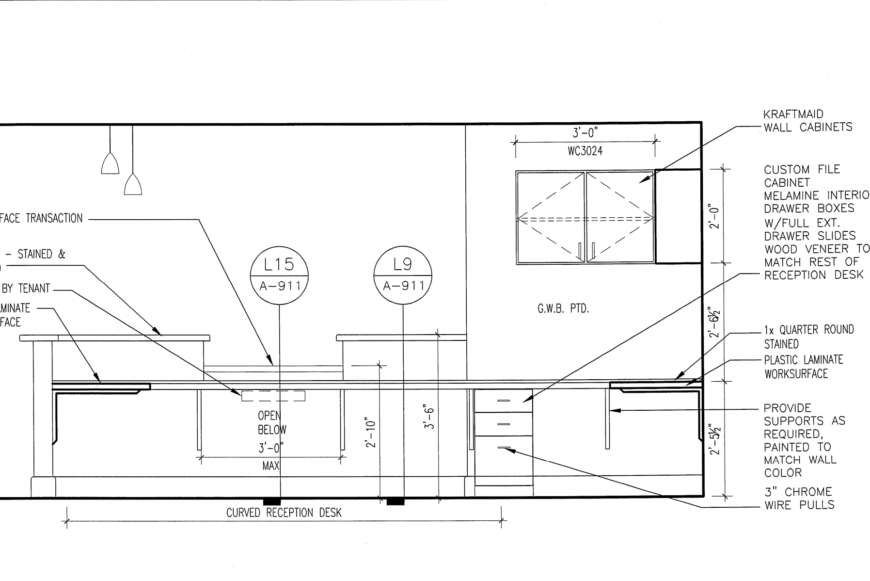
A8 RECEPTION 429 1/2\"/>
