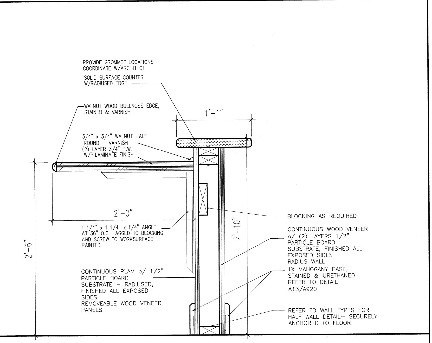
L15 SECTION THRU RECEPTION DESK 1/12\"/>
