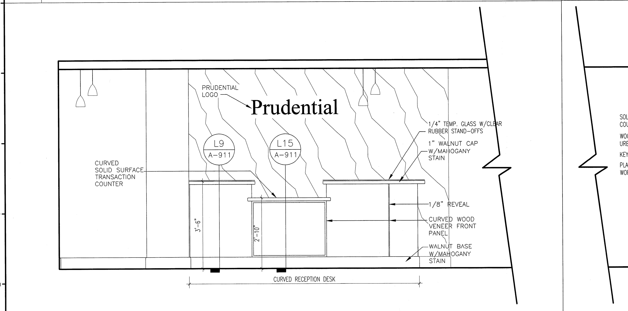
A1 RECEPTION 429 1/2\"/>
