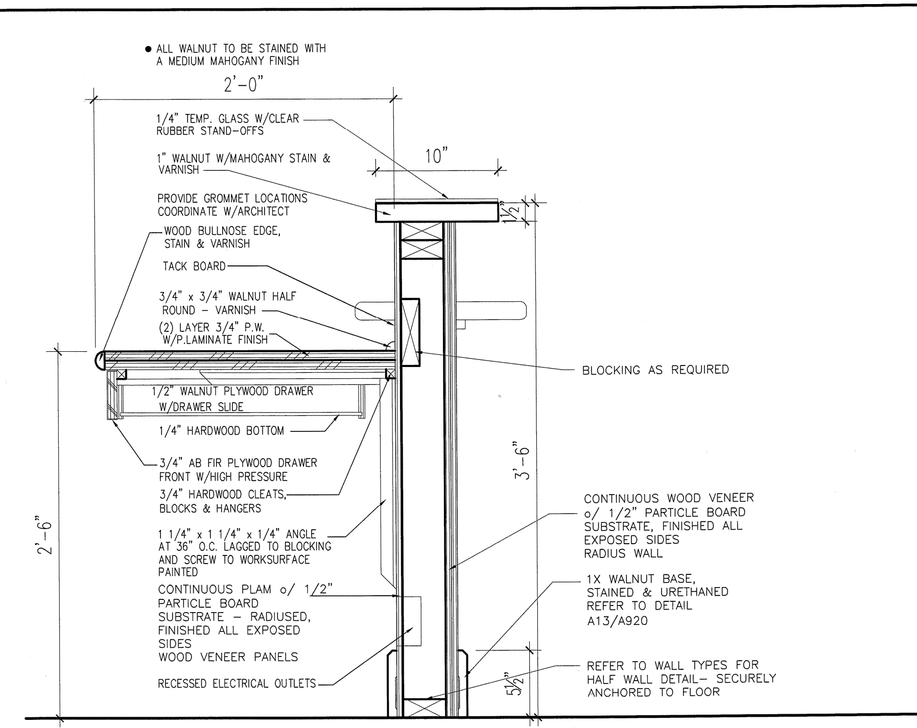
L9 SECTION THRU RECEPTION DESK 1/12\"/>
