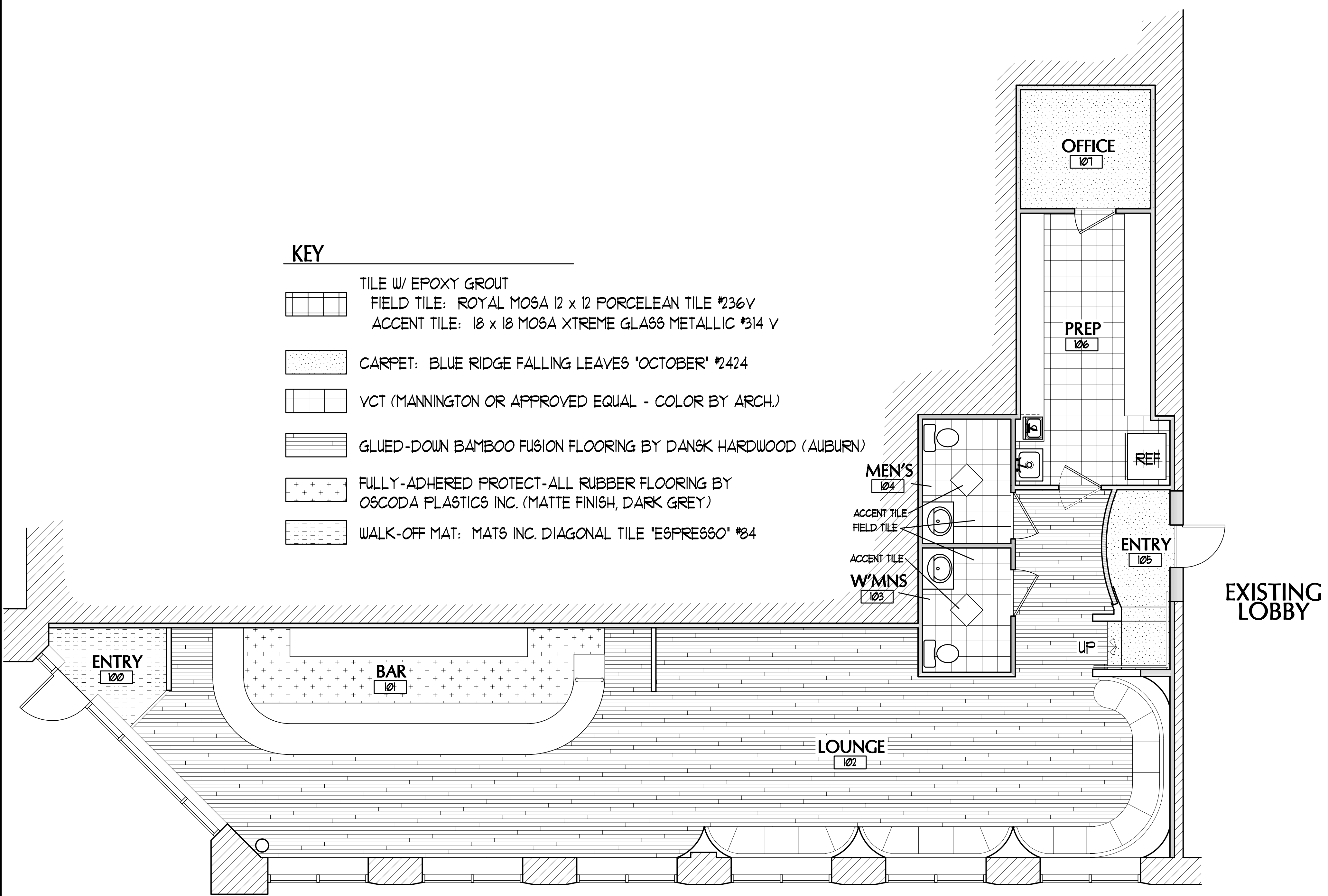
FLOOR FINISHES PLAN SCALE: 1/4" = 1'-0"
