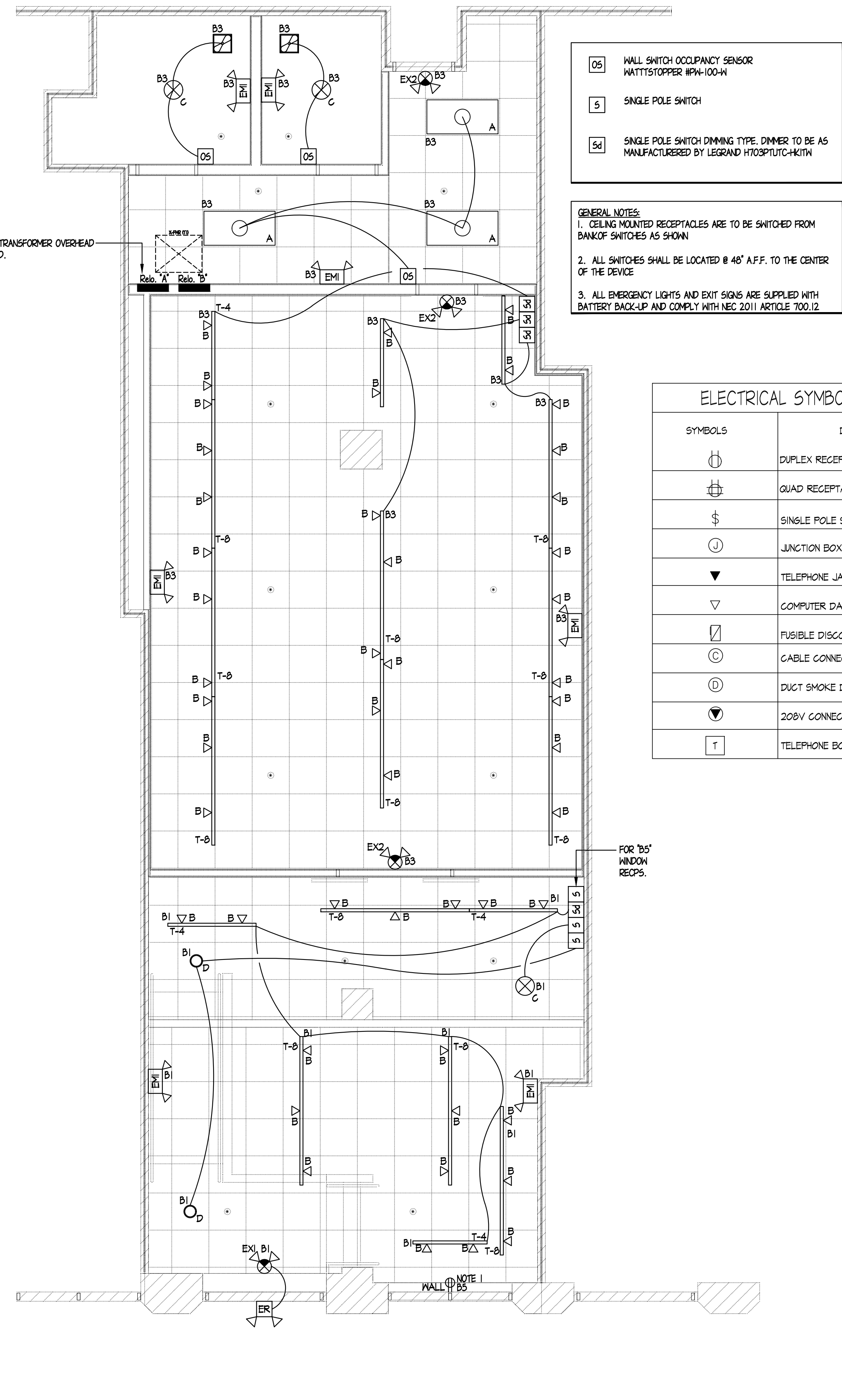
2 LIGHTING PLAN SCALE: 1/4" = 1'-0"
