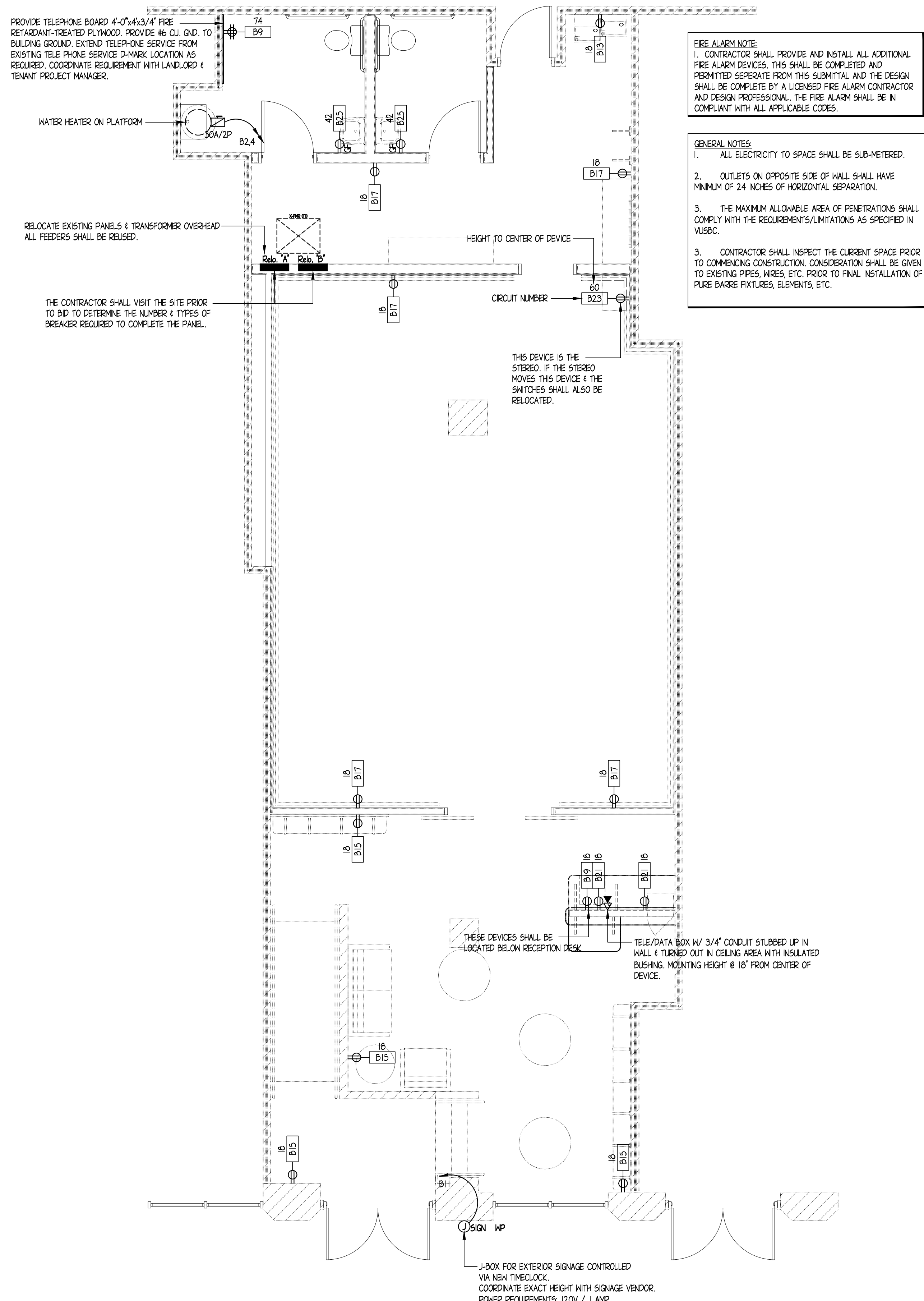
1 POWER PLAN SCALE: 1/4" = 1'-0"
