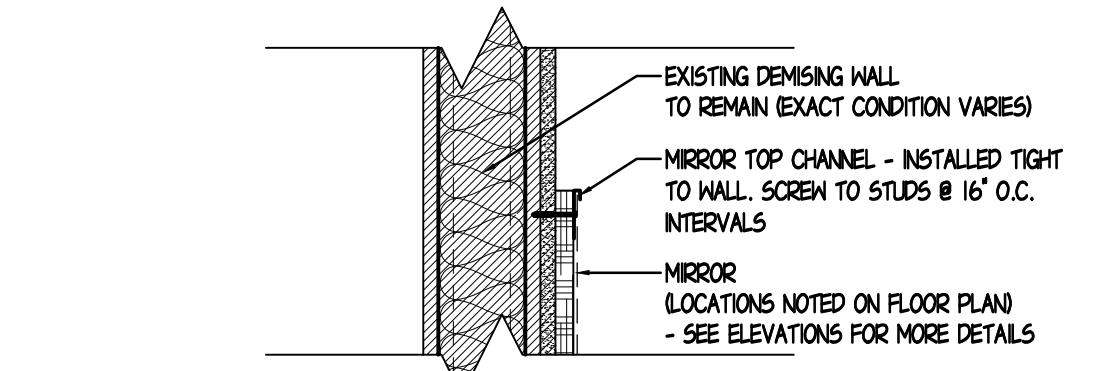
19 TYP. TOP MIRROR BRACKET DETAIL SCALE: 1-1/2" = 1'-0"
