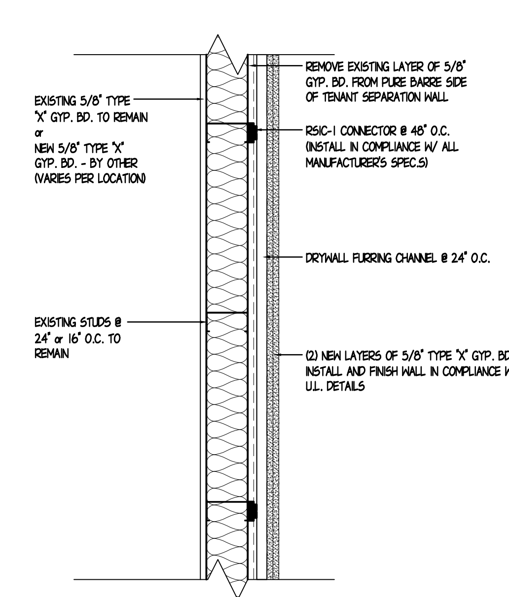
18 ALT. "WORKOUT ROOM" DEMISING WALL DETAIL SCALE: 1-1/2" = 1'-0"
