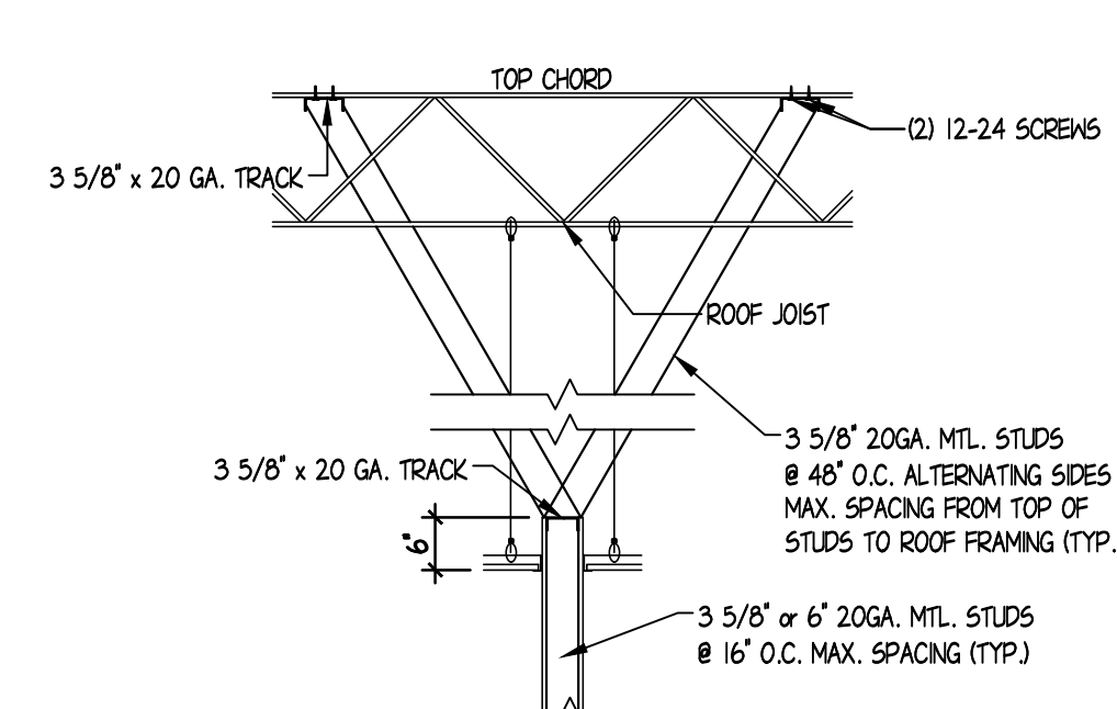
16 TYP. WALL BRACING DETAIL NOT TO SCALE
