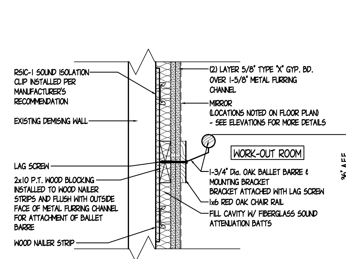
21 ALT. "WORKOUT ROOM" DEMISING WALL DETAIL SCALE: 1-1/2" = 1'-0"
