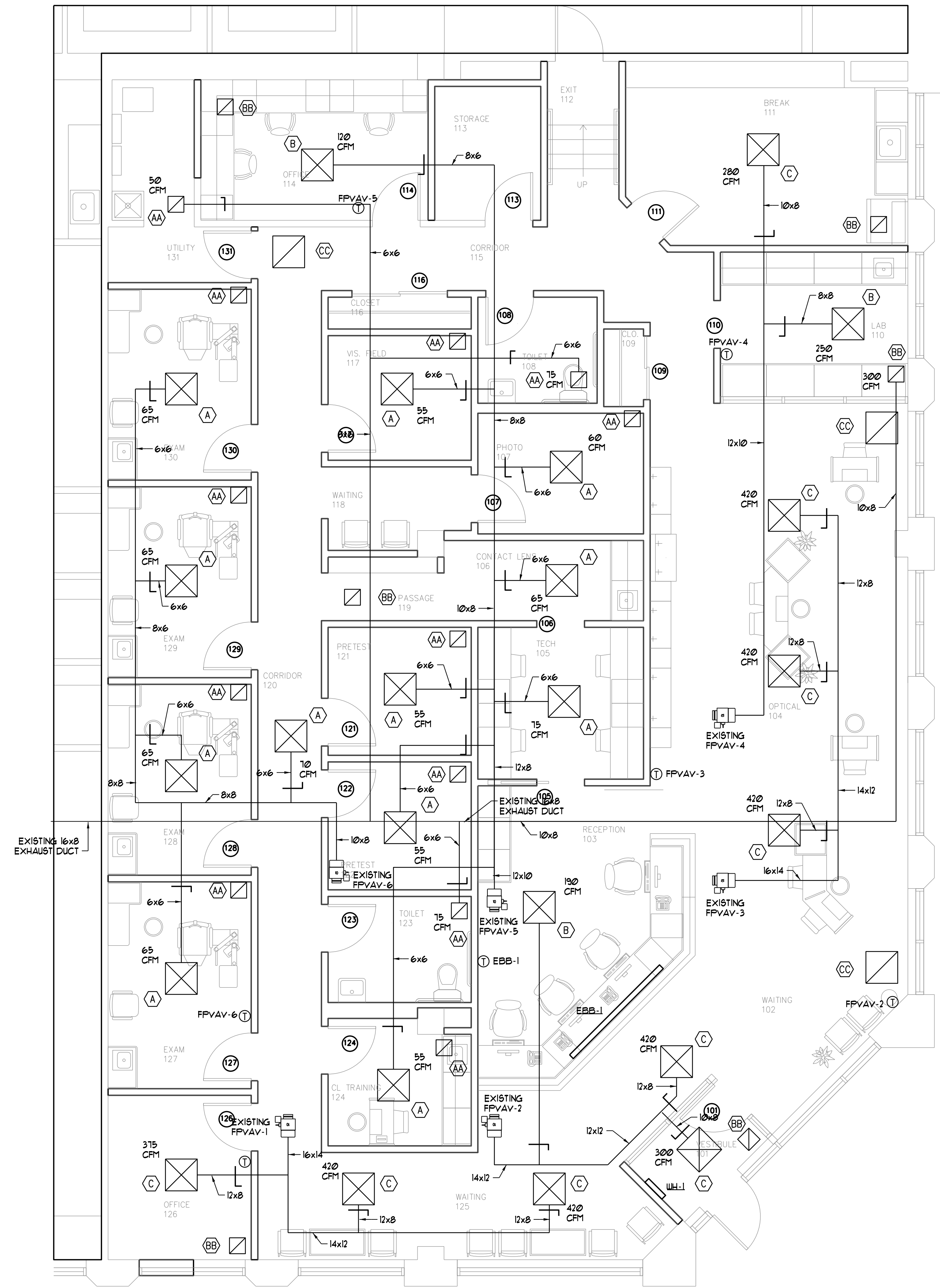
MECHANICAL PLAN SCALE - 1/4" = 1'-0"
