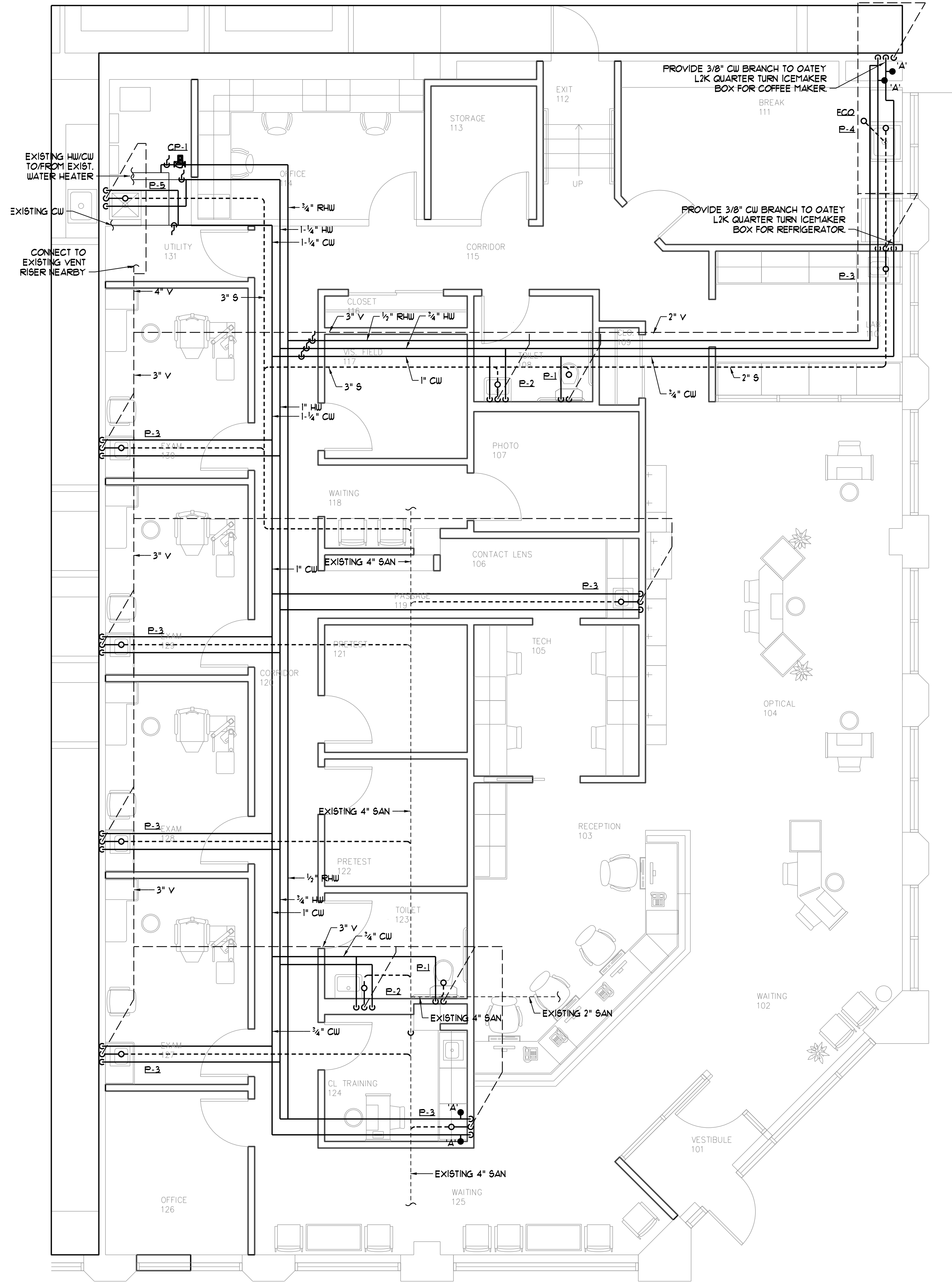
PLUMBING PLAN SCALE - 1/4" = 1'-0"
