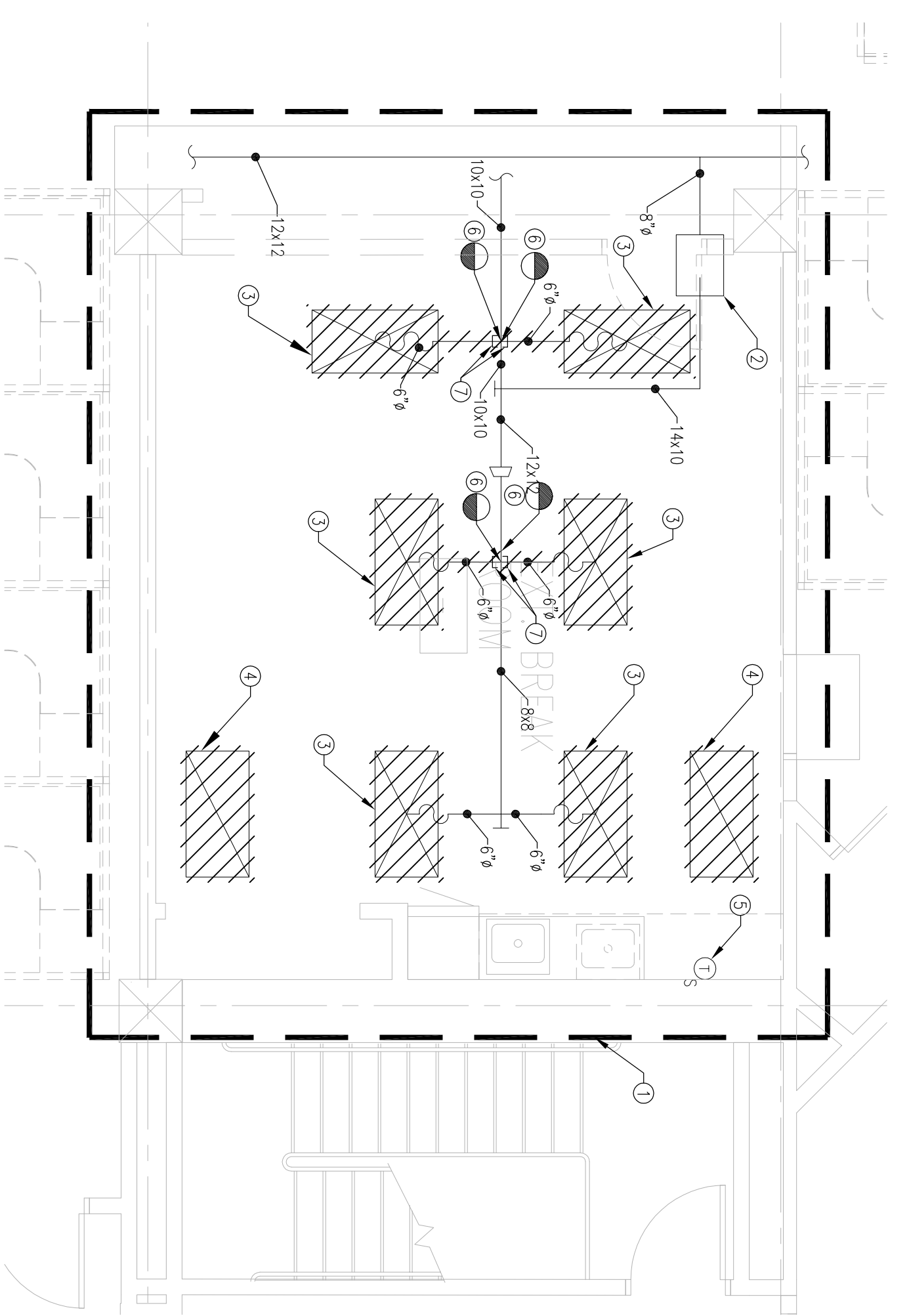
1 7TH FLOOR PLAN - DEMO HVAC SCALE: 1/4"=1'-0"
