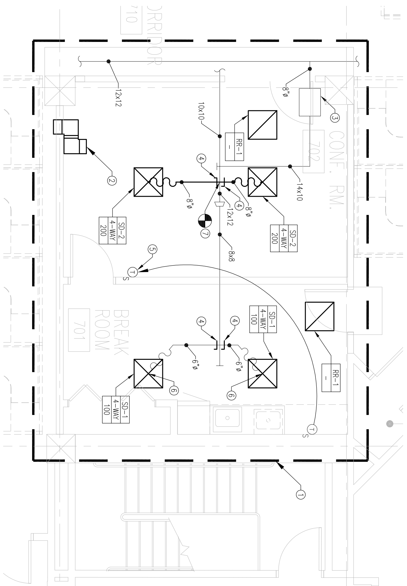
2 7TH FLOOR PLAN - HVAC SCALE: 1/4"=1'-0"
