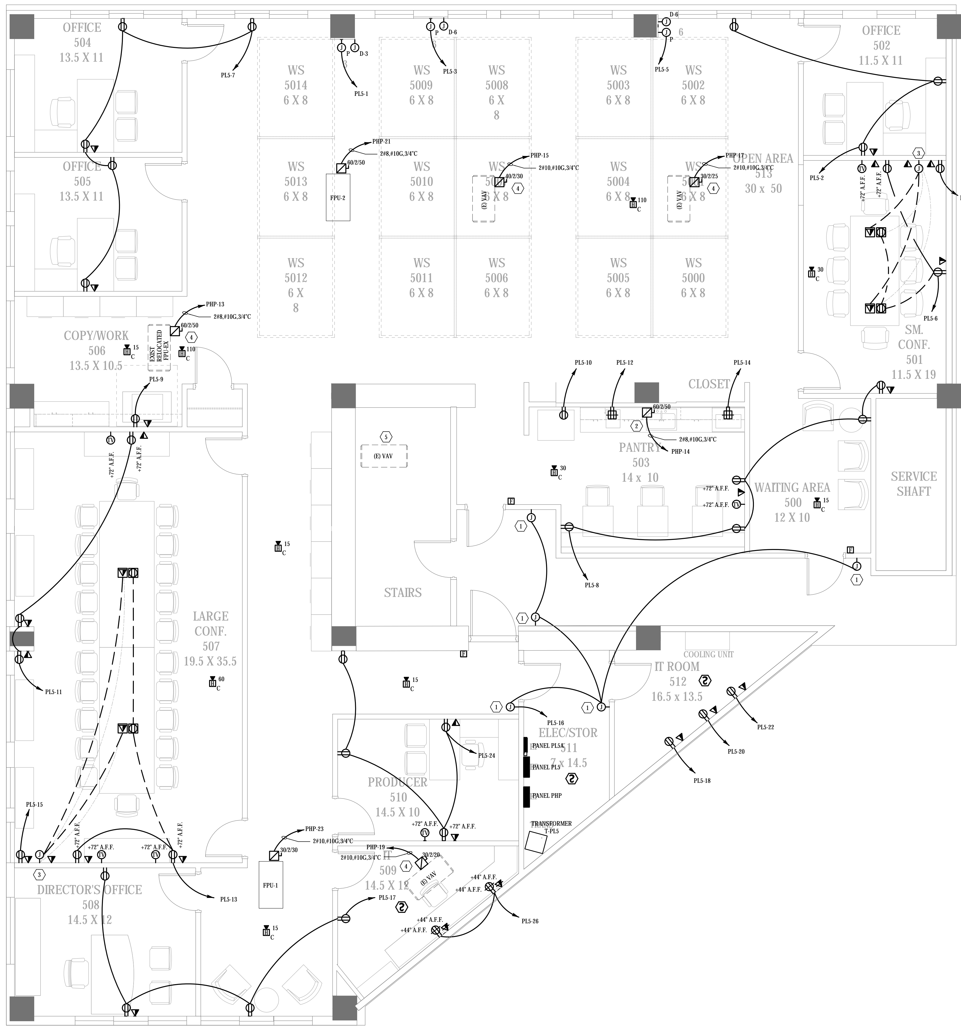
1 ELECTRICAL POWER FLOOR PLAN SCALE: 1/4" = 1'-0"
