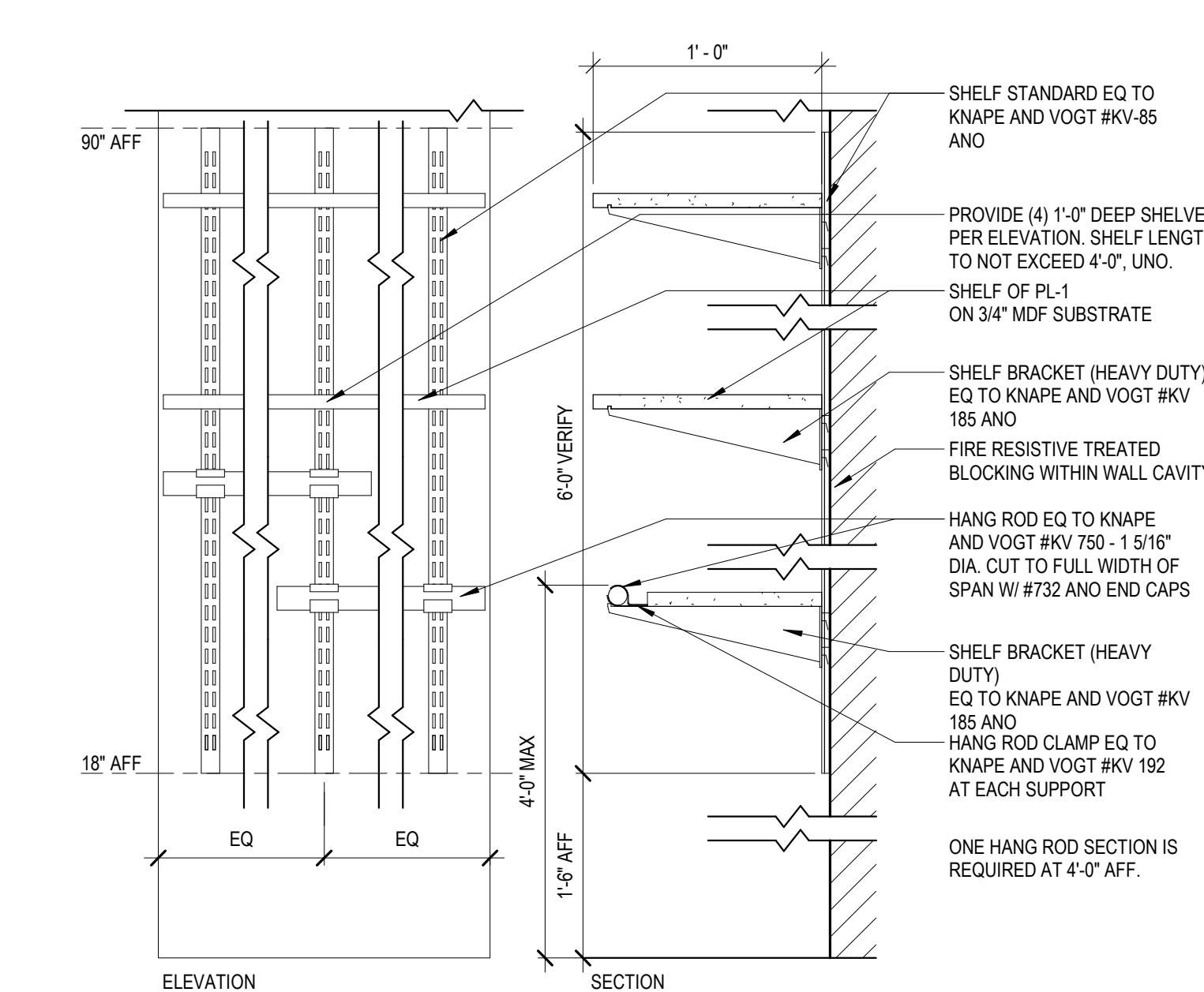
C3 DETAIL @ ROD AND SHELF SCALE: 1 1/2" = 1'-0"
