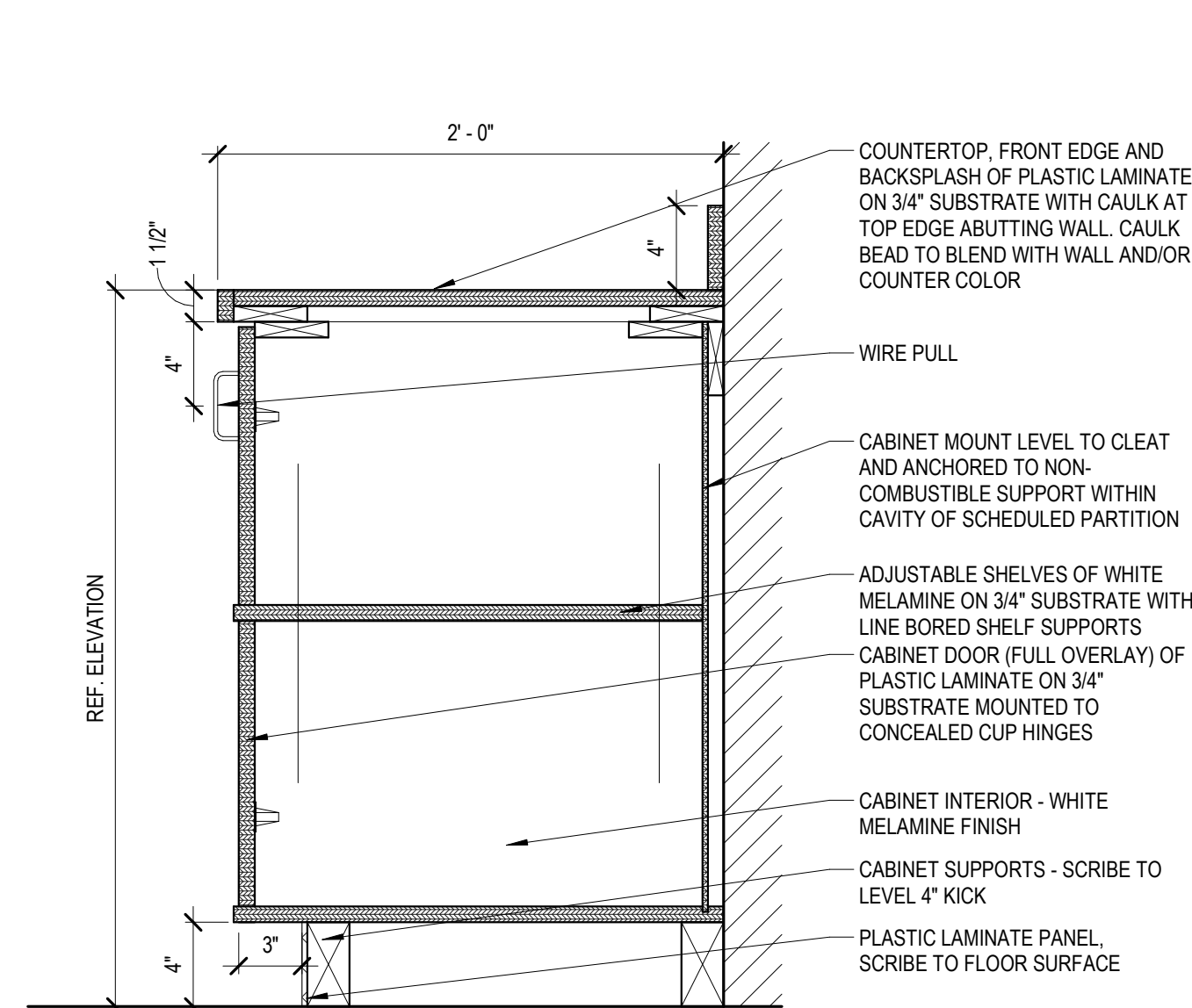
C2 MILLWORK DETAIL SCALE: 1 1/2" = 1'-0"
