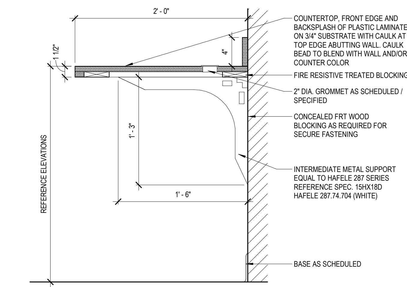
B2 MILLWORK DETAIL SCALE: 1 1/2" = 1'-0"
