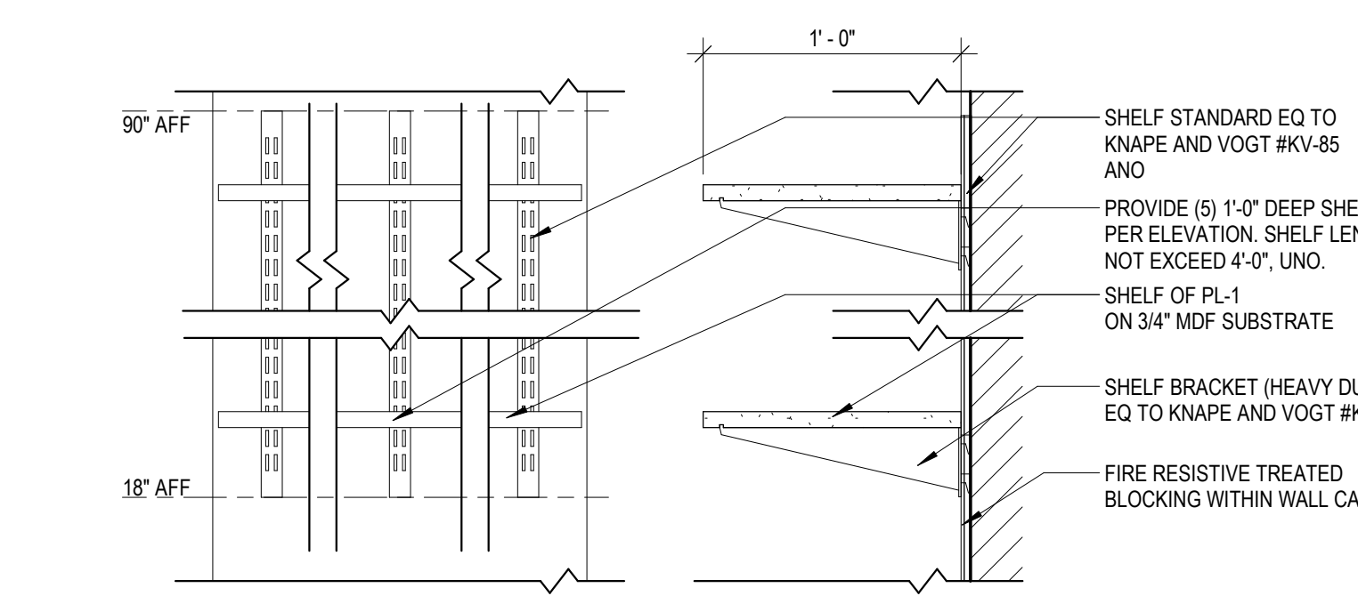
C4 DETAIL @ ADJUSTABLE SHELVES SCALE: 1 1/2" = 1'-0"
