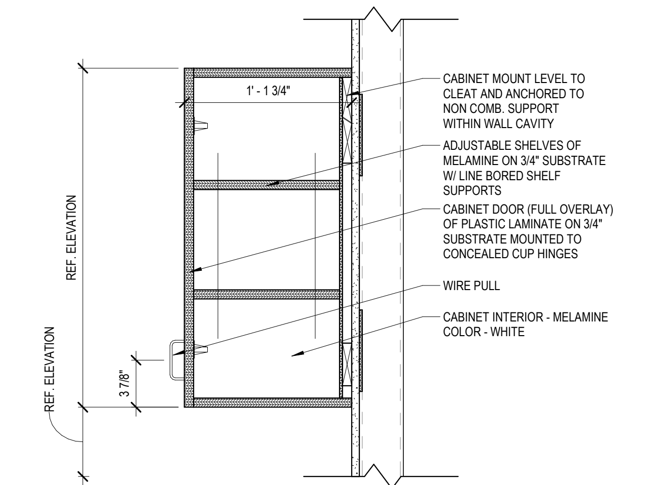
B1 MILLWORK DETAIL SCALE: 1 1/2" = 1'-0"
