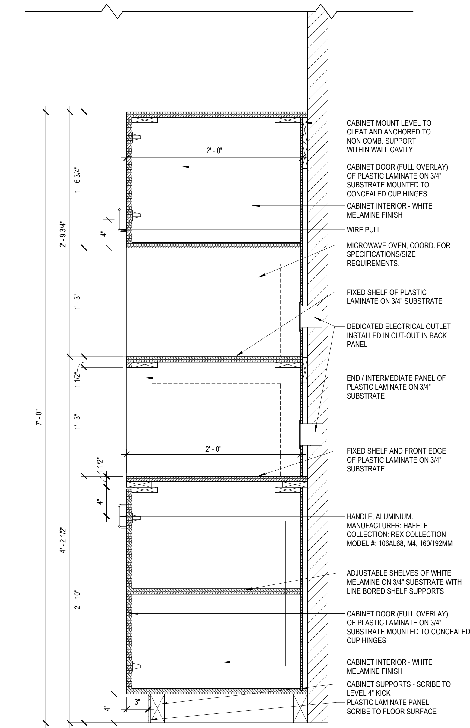
B4 MILLWORK DETAIL SCALE: 1 1/2" = 1'-0"
