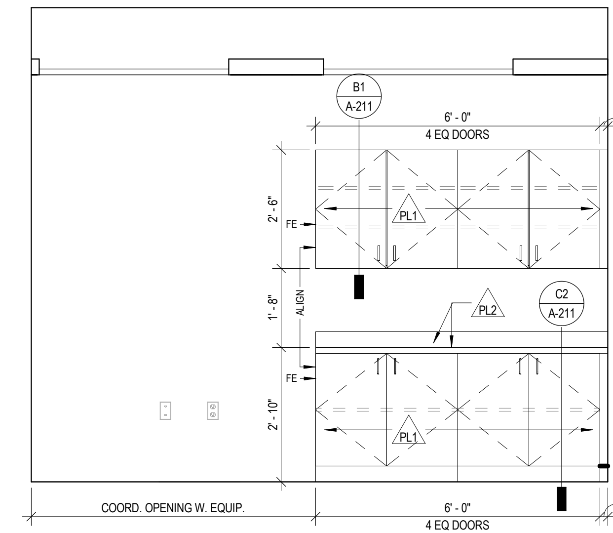
D3 ELEVATION @ COPY/WORK 506 SCALE: 1/2" = 1'-0"
