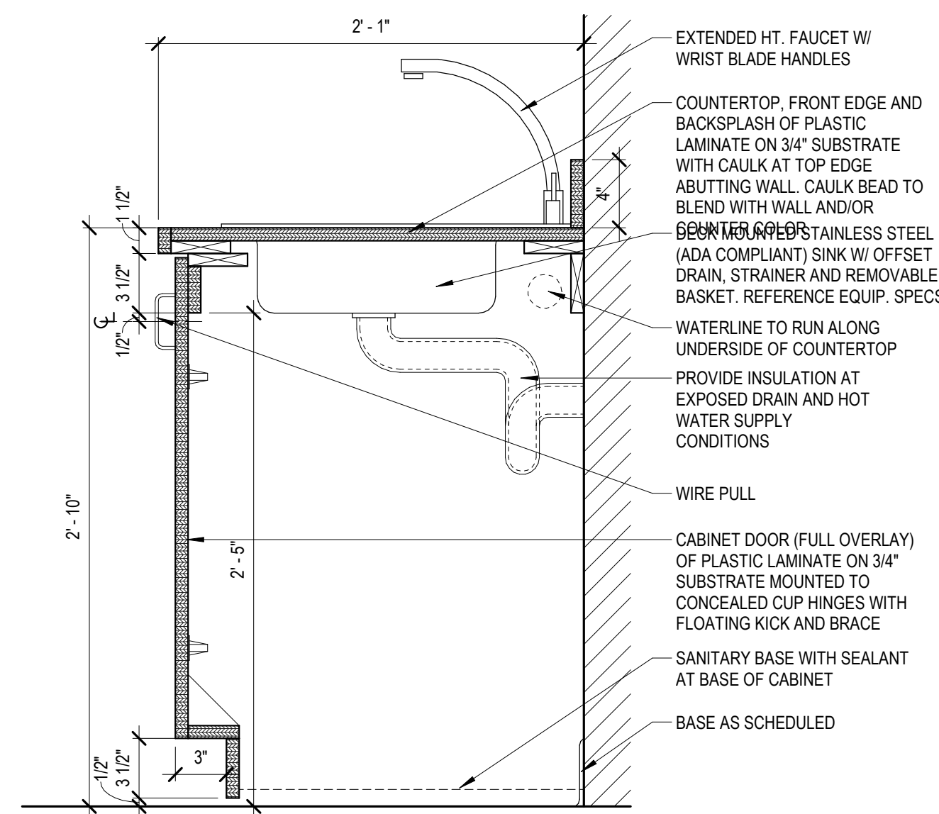
C1 MILLWORK DETAIL SCALE: 1 1/2" = 1'-0"
