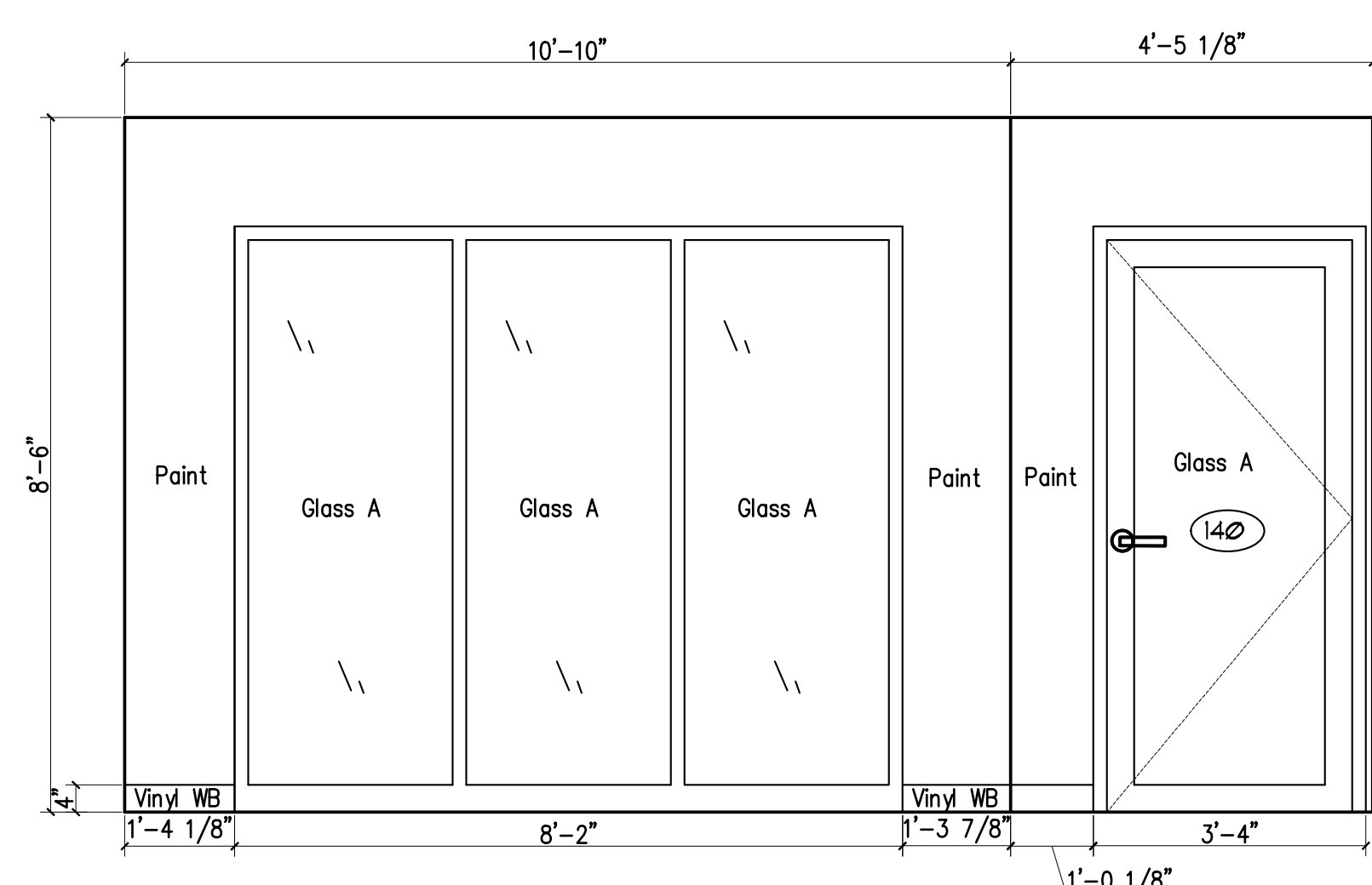
11 OFFICE 140 - ELEVATION 1/2" = 1'-0"
