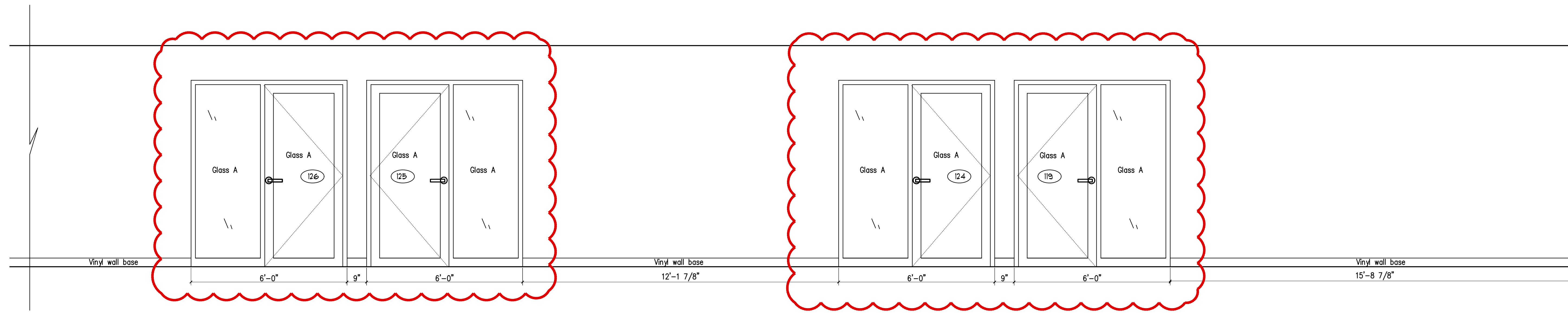
7B NEW EXTERIOR OFFICE FRONTS - (PARTIAL) ELEVATION 1/2" = 1'-0"
