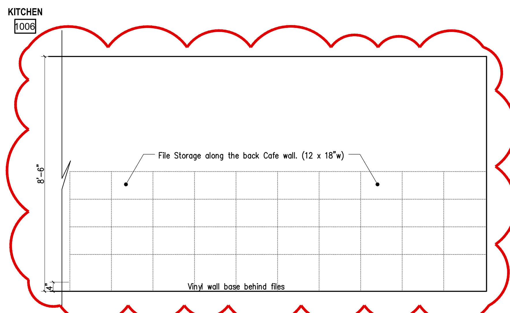
8 CAFE 143 - ELEVATION 1/2" = 1'-0"
