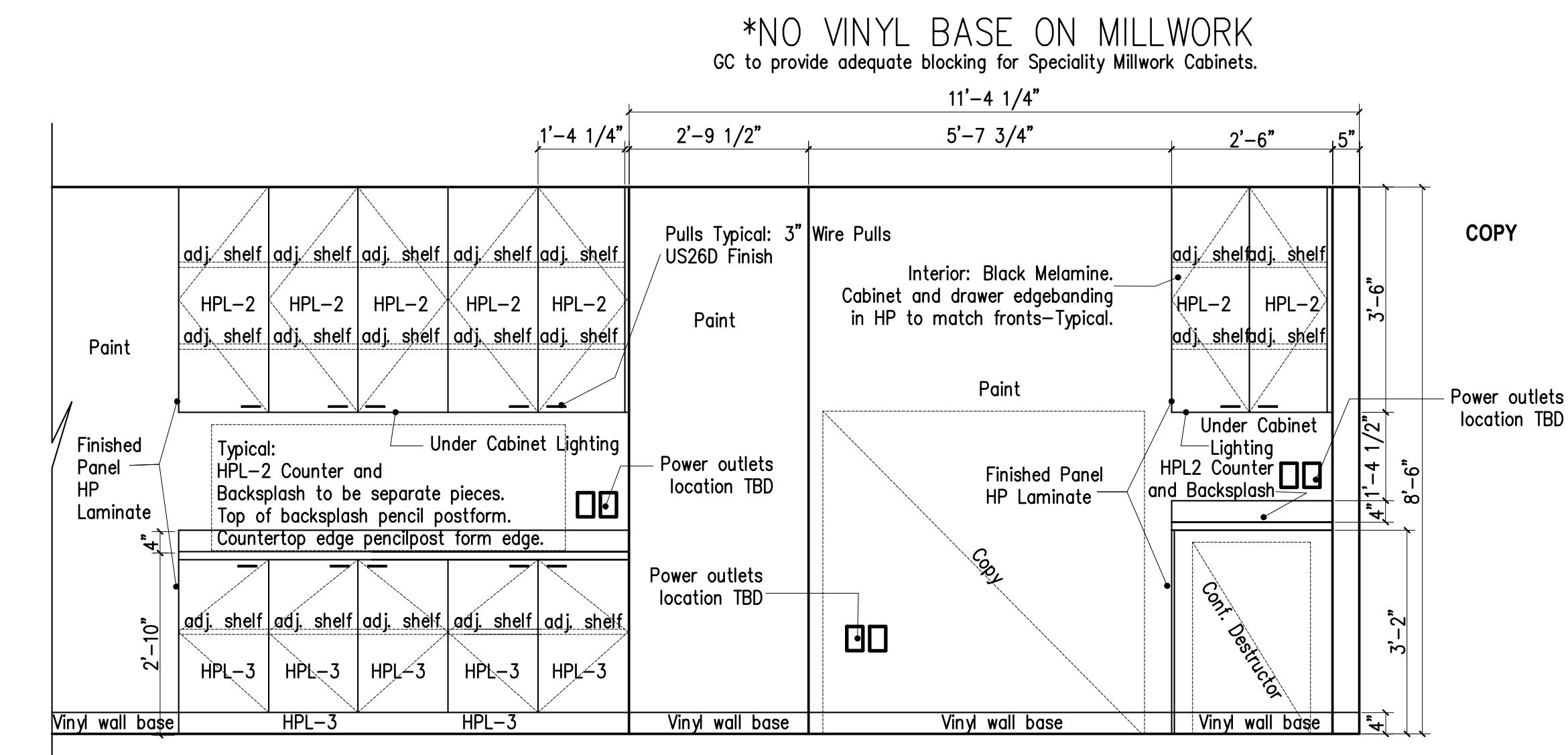
10 COPY 146 - ELEVATION 1/2" = 1'-0"
