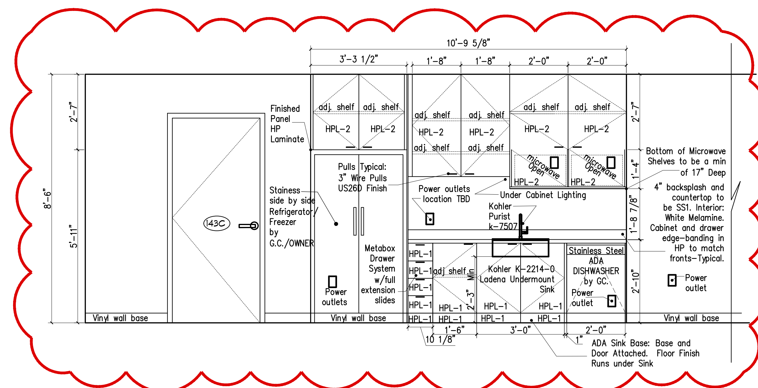
9 CAFE 143 - ELEVATION 1/2" = 1'-0"
