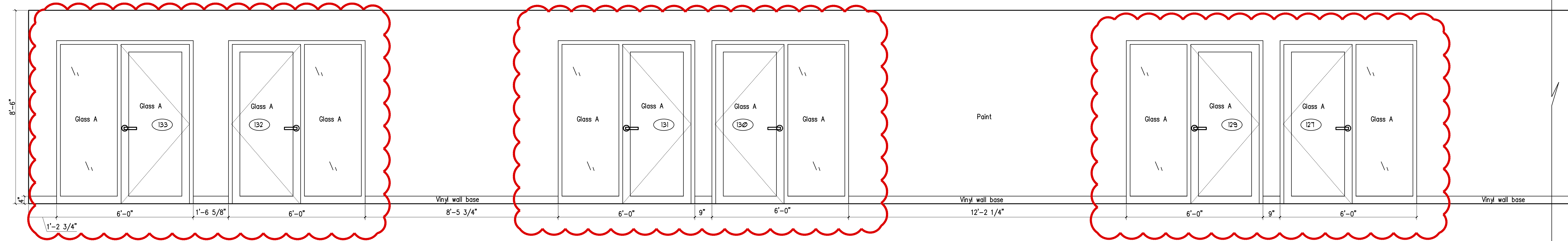
7A NEW EXTERIOR OFFICE FRONTS - (PARTIAL) ELEVATION 1/2" = 1'-0"
