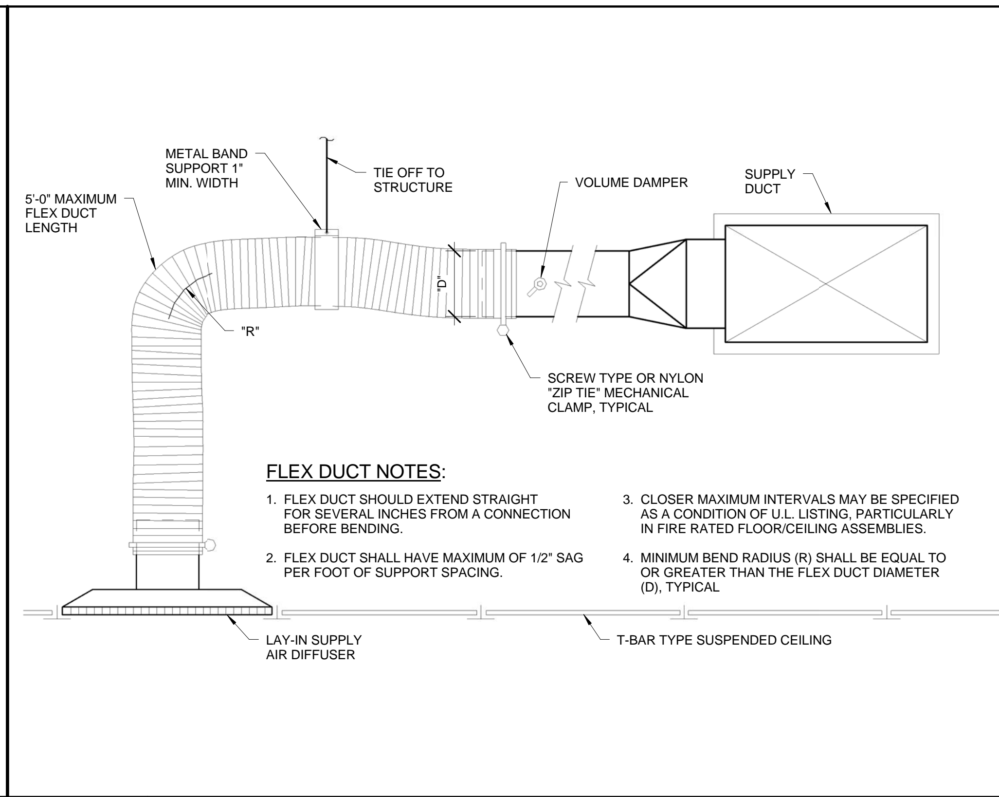
E5 DETAIL - SUPPLY AIR BRANCH CONNECTION
