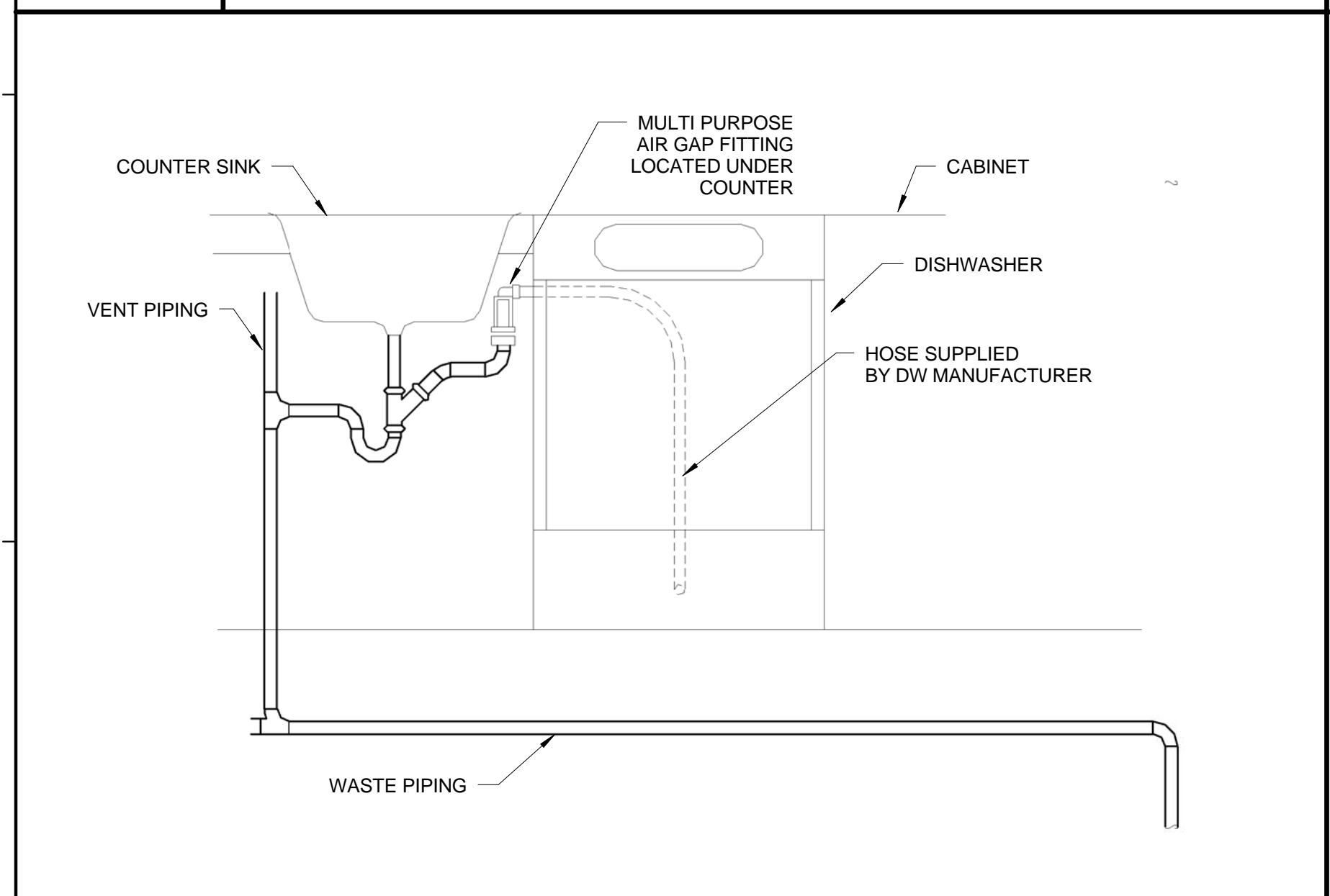
A1 DETAIL - SINK AND DISHWASHER
