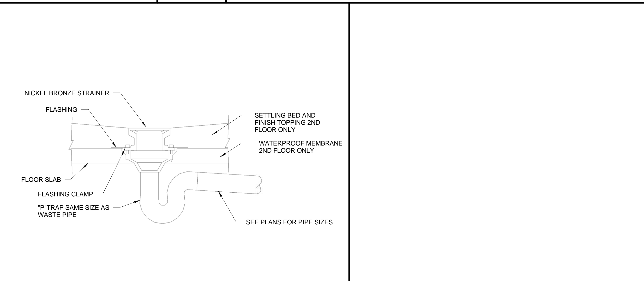
C4 FLOOR DRAIN DETAIL
