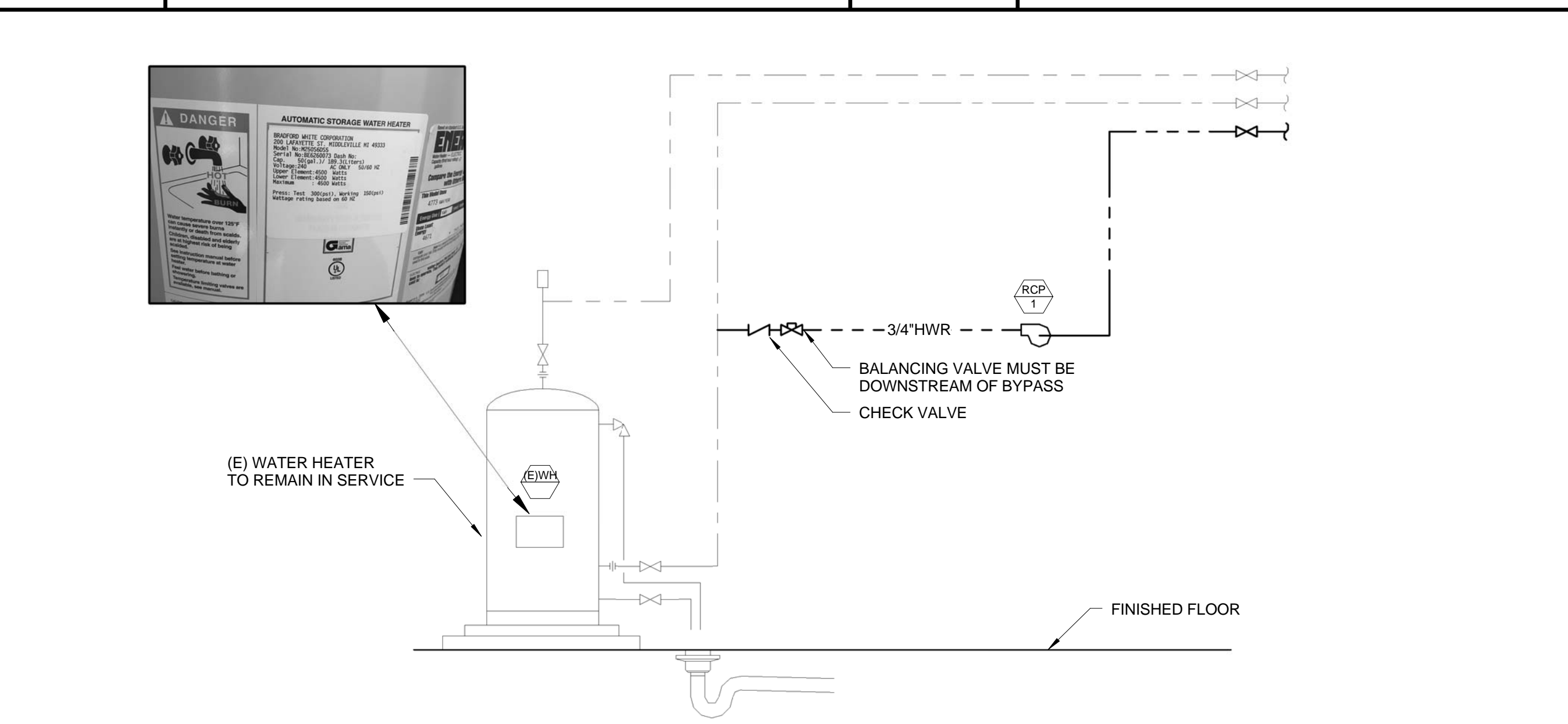
A4 DETAIL - ELECTRIC WATER HEATER
