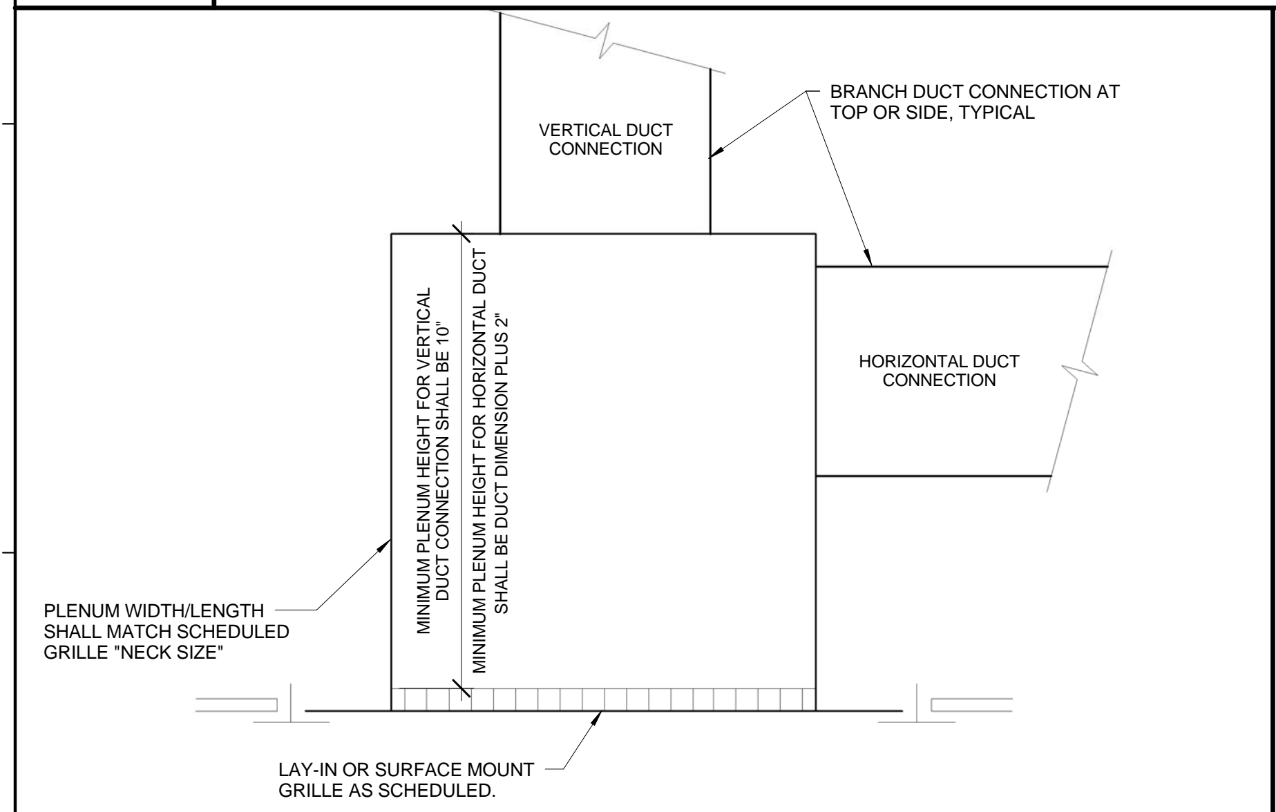
C1 DETAIL - SUPPLY/RETURN AIR REGISTER BOOT
