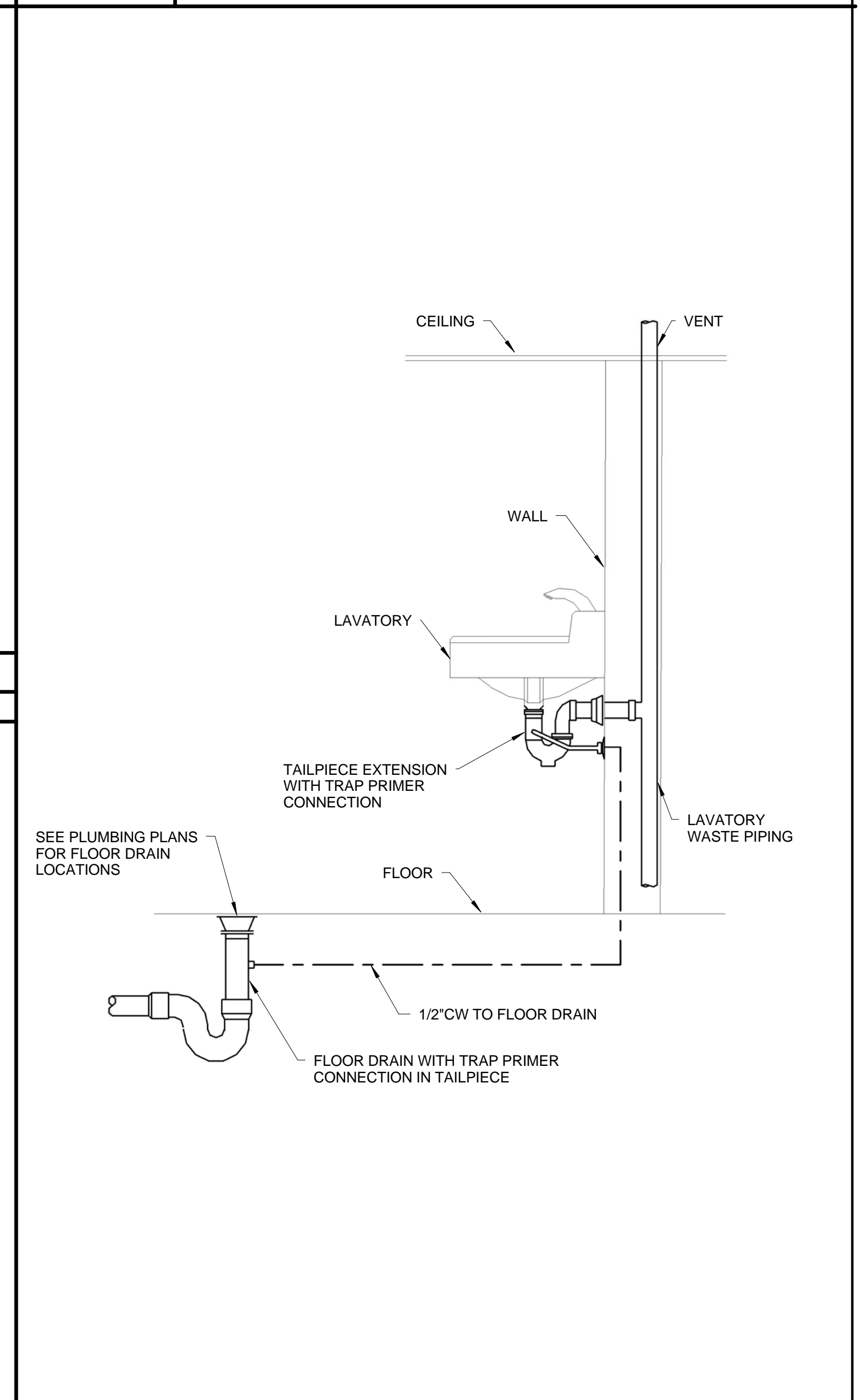
A8 DETAIL - WATER SVER TRAP PRIMER DETAIL TP-1
