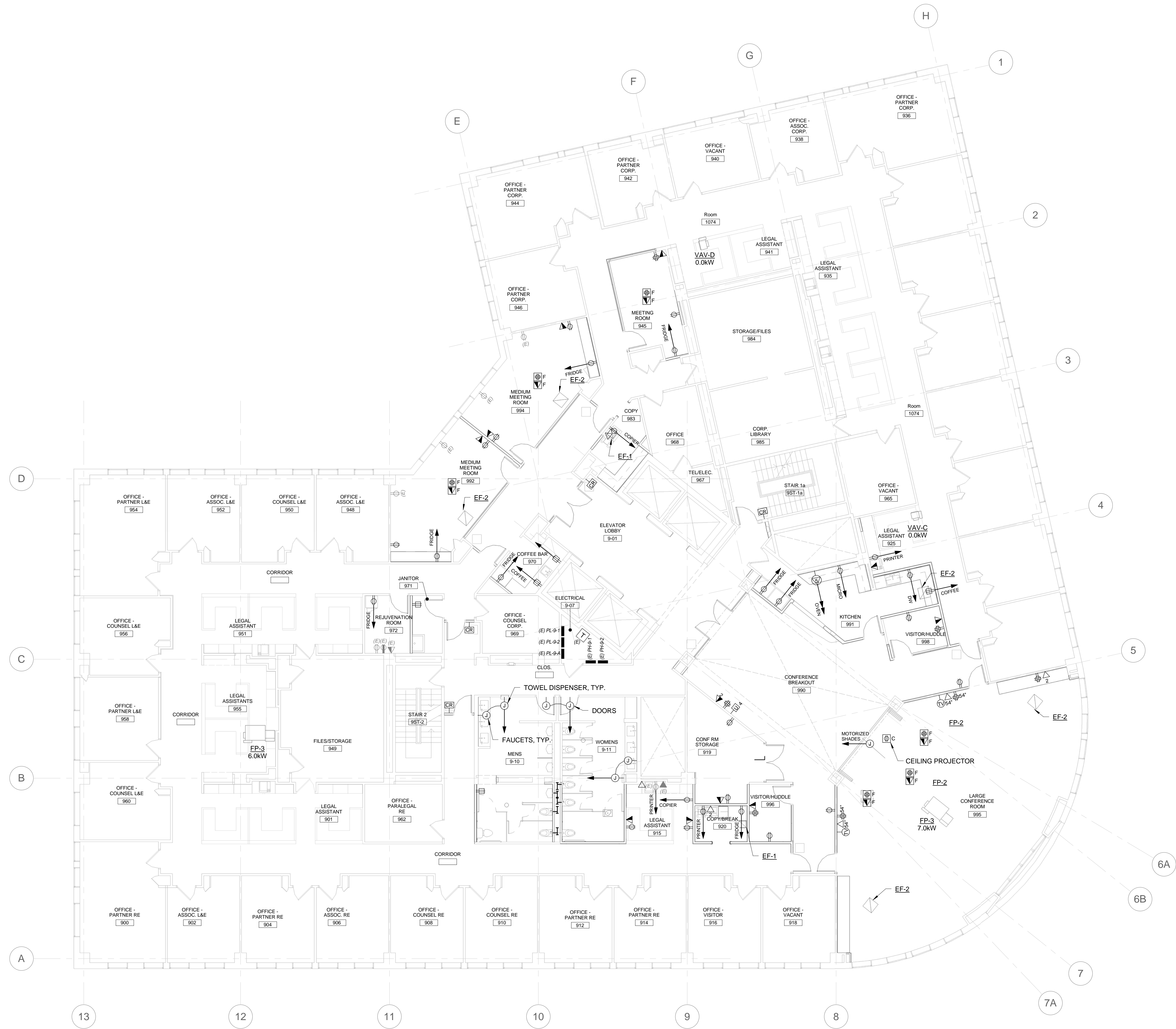
A1 FLOOR 9 POWER AND SYSTEMS PLAN 1/8" = 1'-0"
