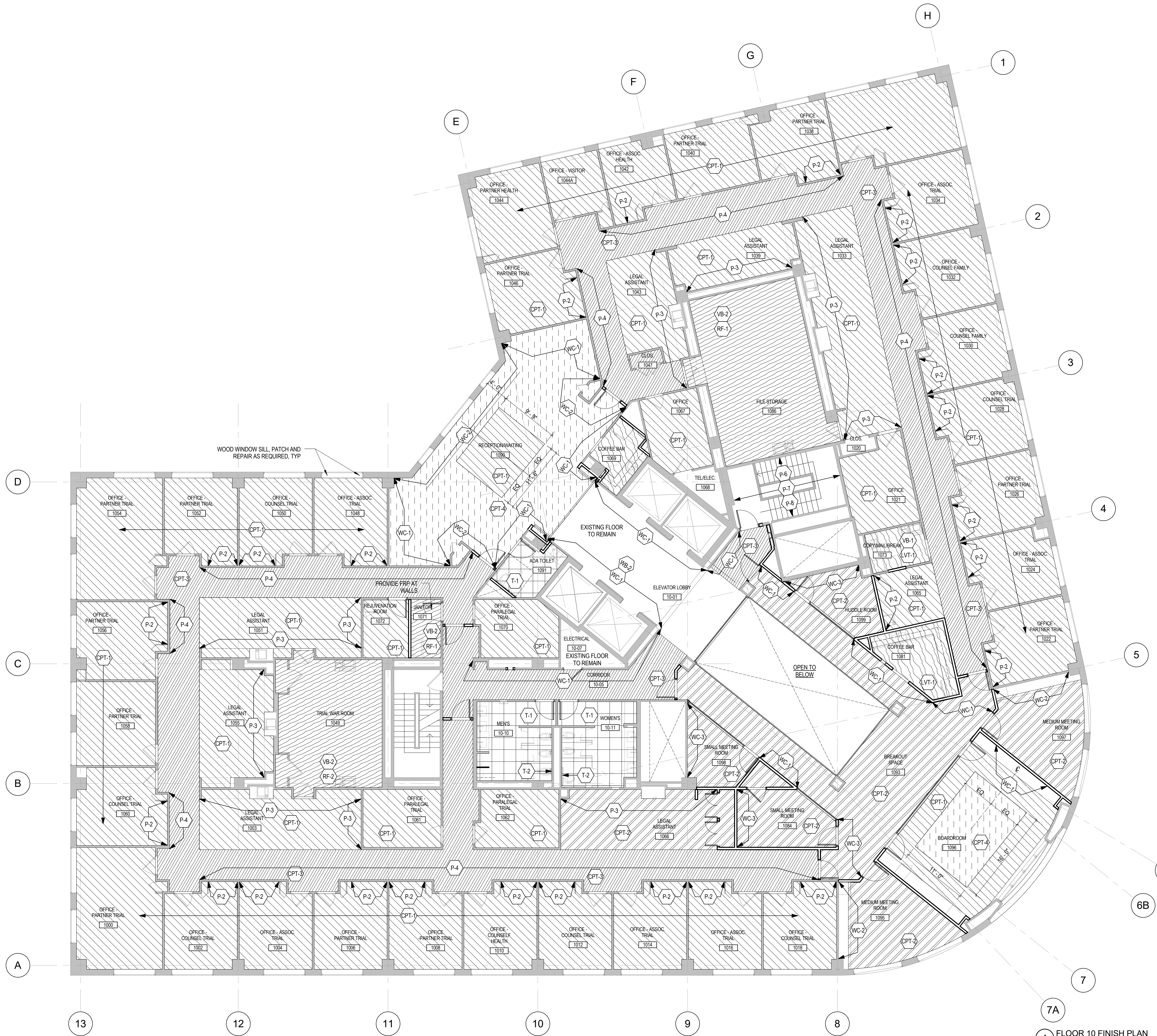
FLOOR 10 FINISH PLAN 1/8" = 1'-0"
