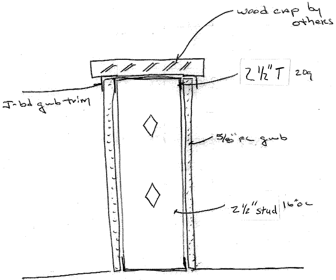
Low Wall Framing Detail note Hts. may vary.
