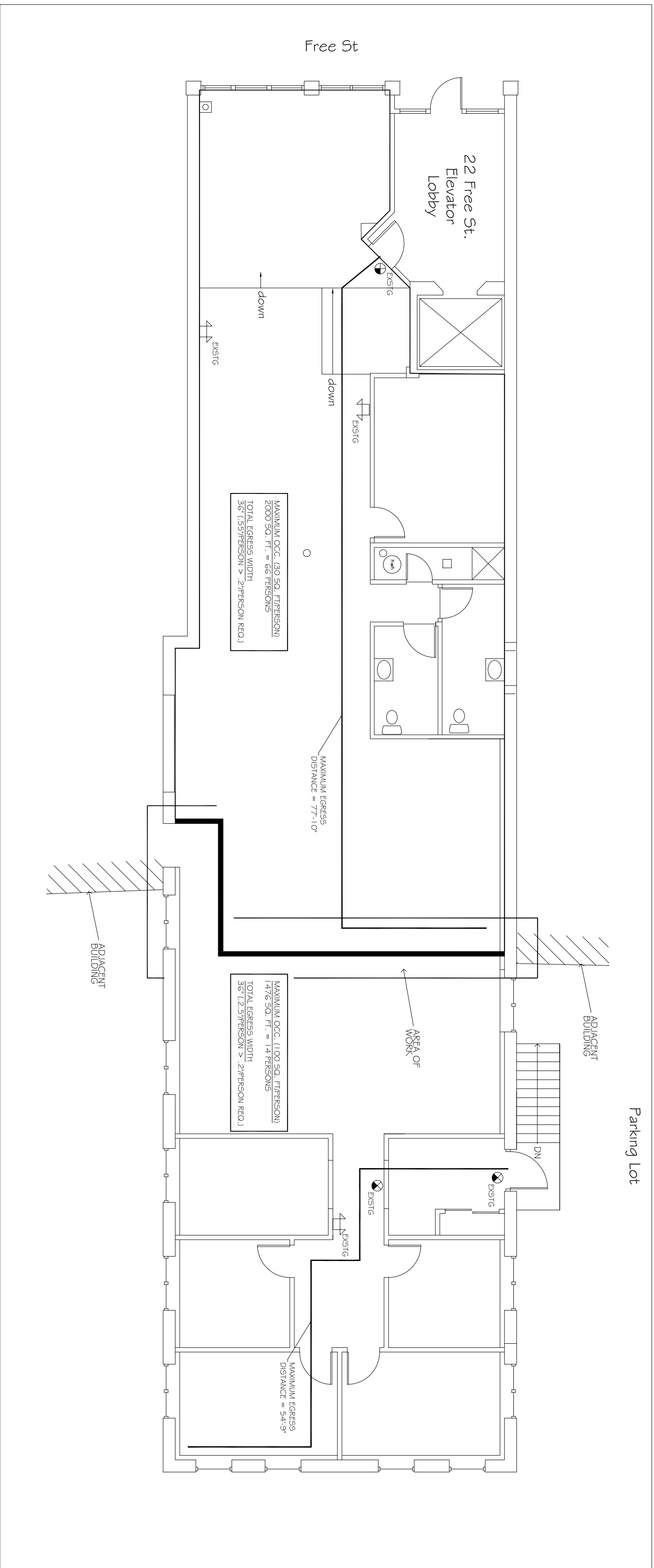
A1 EGRESS PLAN 1/8" = 1'-0"
