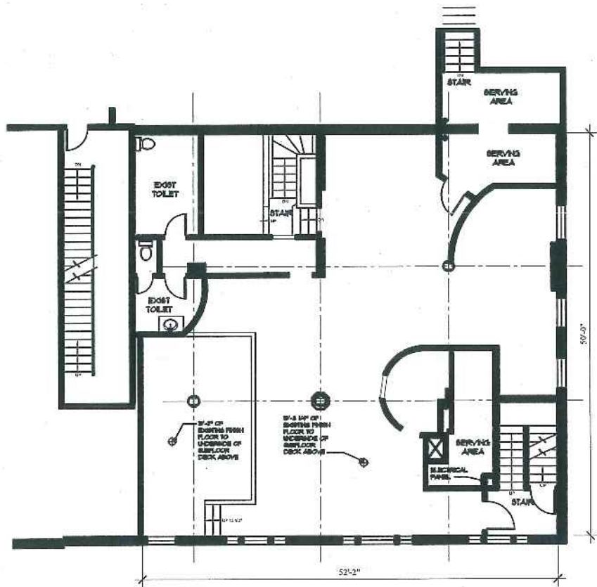
2nd FLOOR
