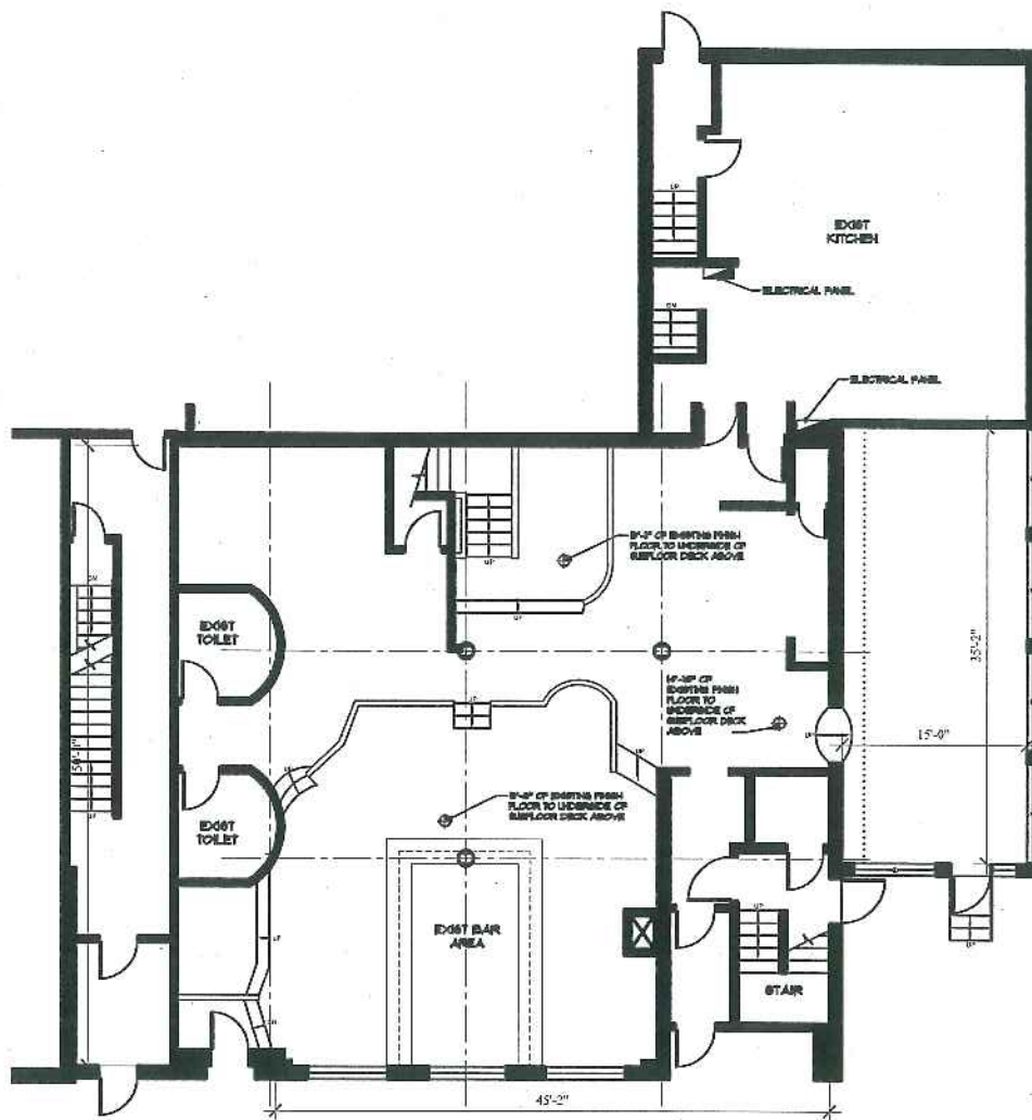
1st FLOOR
