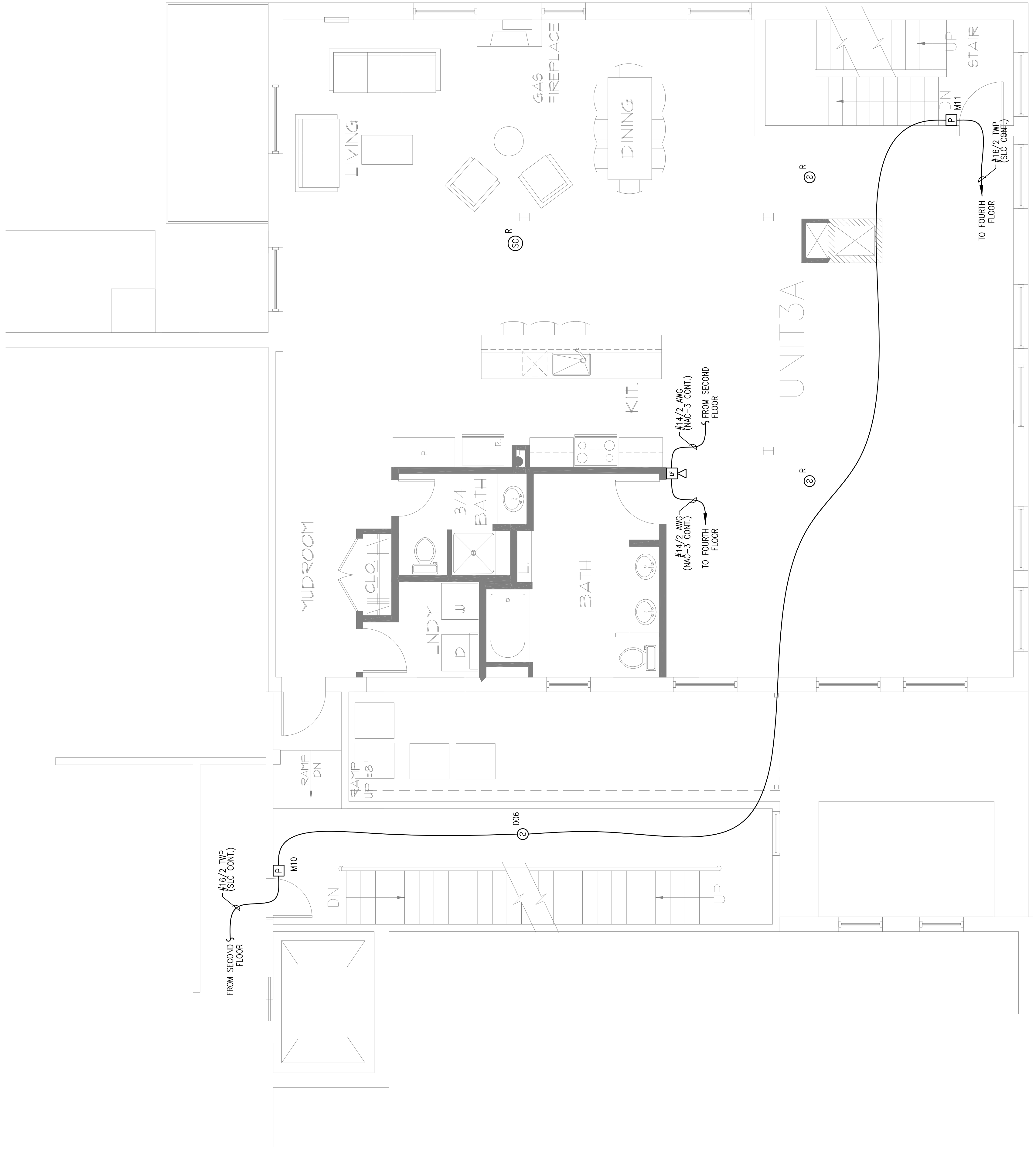
PLAN WITH THIRD FLOOR FIRE ALARM PLAN SCALE: 1/4"=1'-0"
