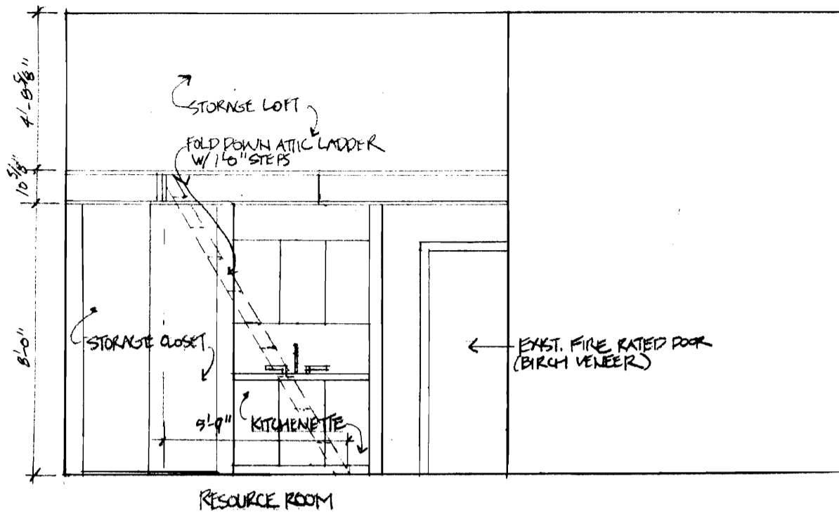
ELEVATION C SCALE = 1/4" = 1'-0"
