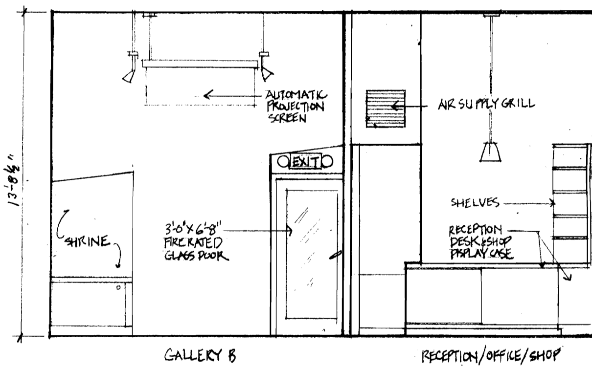
ELEVATION B SCALE = 1/4" = 1'-0"
