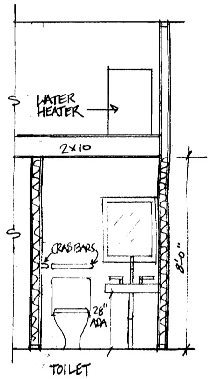
ELEVATION D SCALE = 1/4" = 1'-0"
