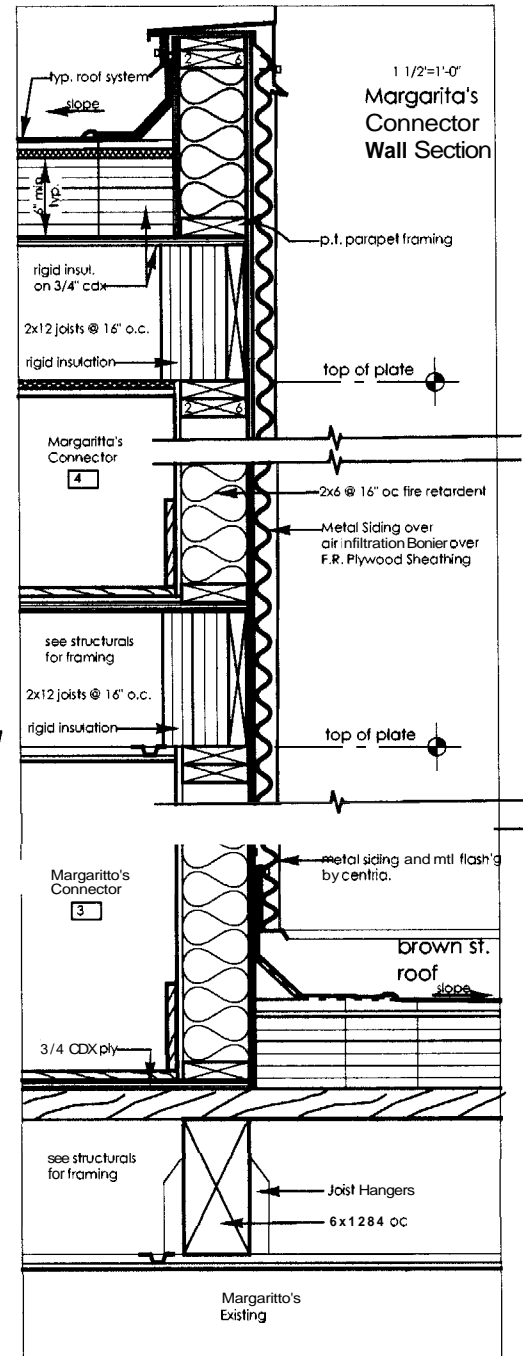
SECTION THRU NEW CONNECTOR 1 1/2" = 1' - 0"
