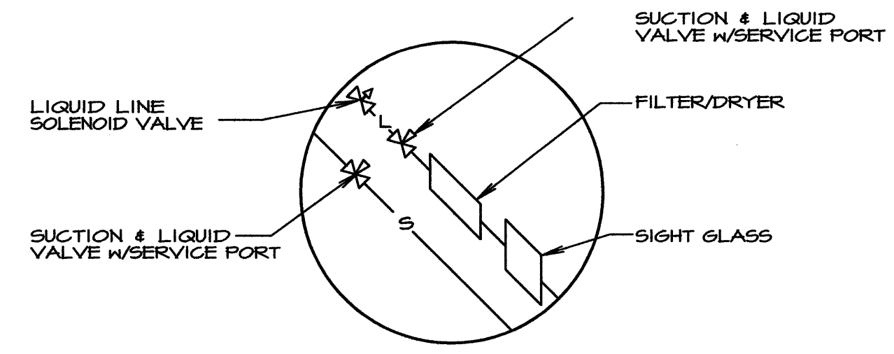
CONDENSING UNIT PIPE CONNECTION NO SCALE
