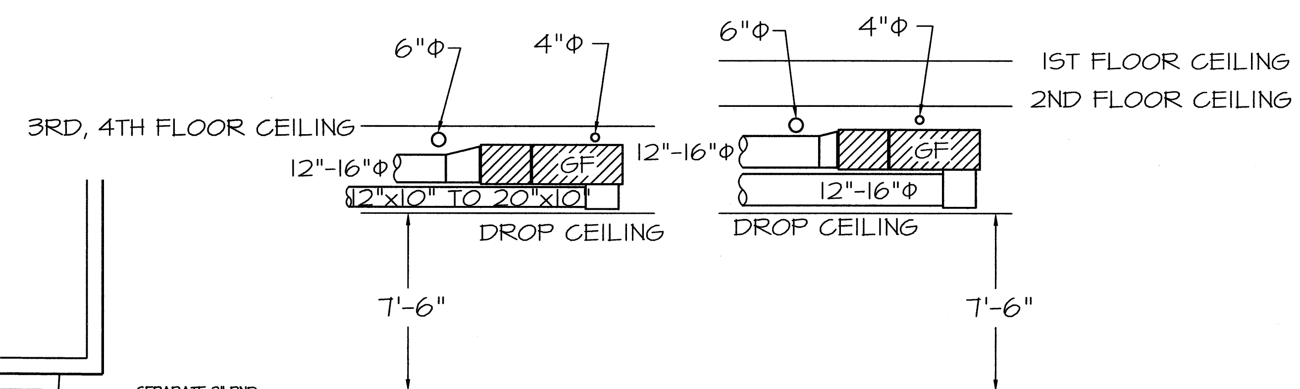
FLOOR FLOOR GAS FURNACE DUCTWORK CLEARANCE DETAIL NO SCALE
